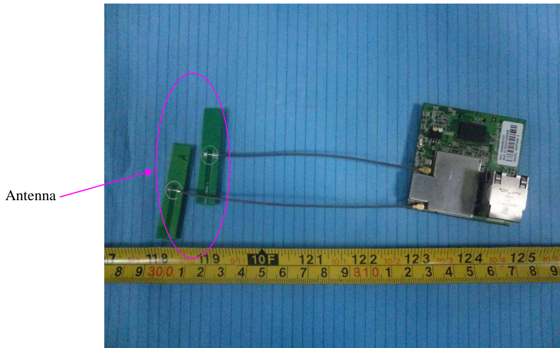
EUT -Front with Antenna View
