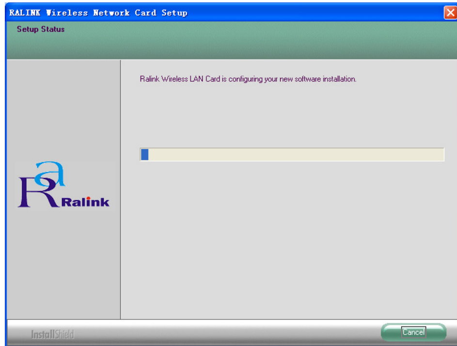
Figure 2-2 Start Setup
