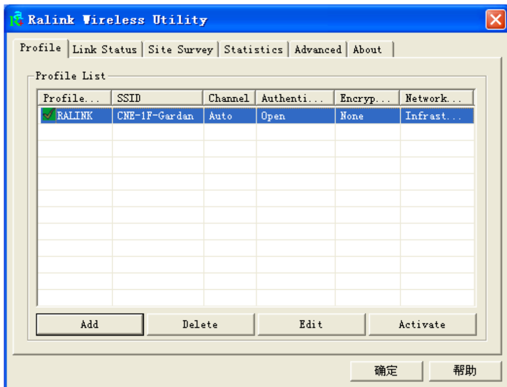
Figure 3-1 Profile Tab
