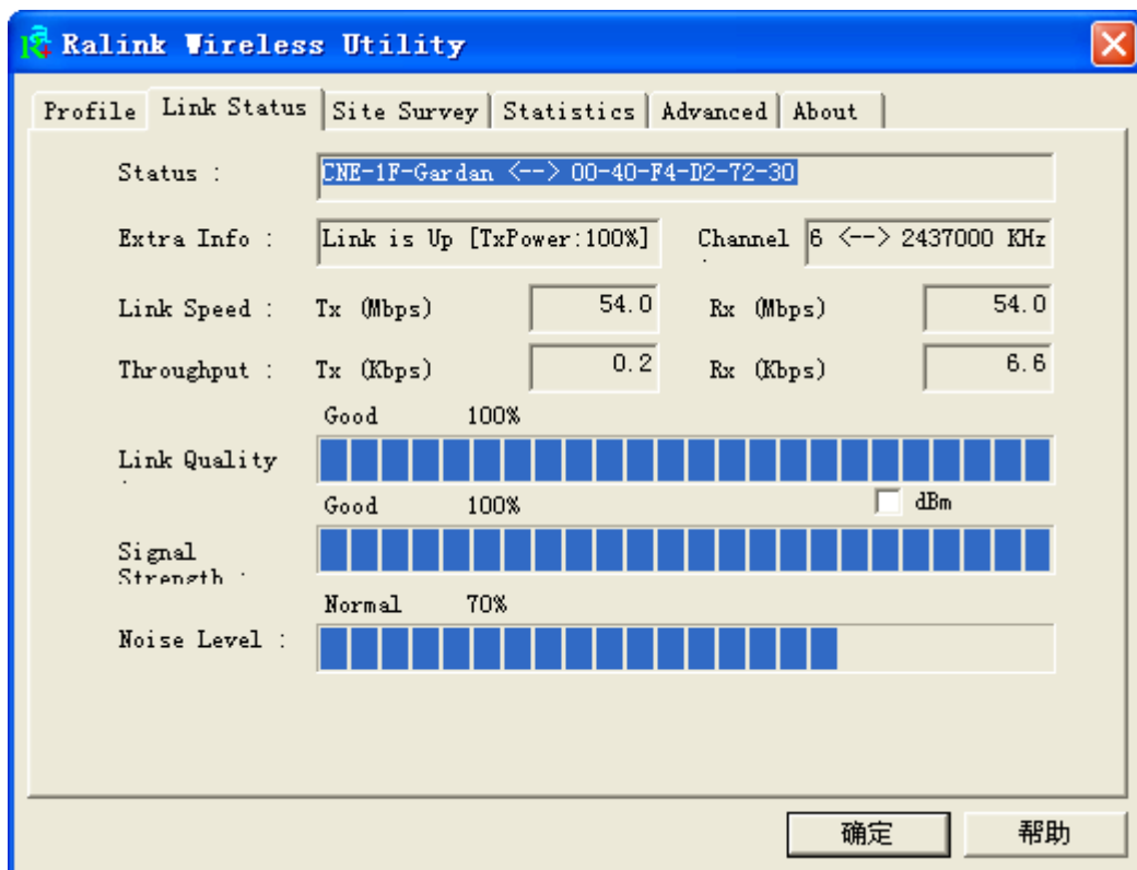
Figure 3-4 Link Status
