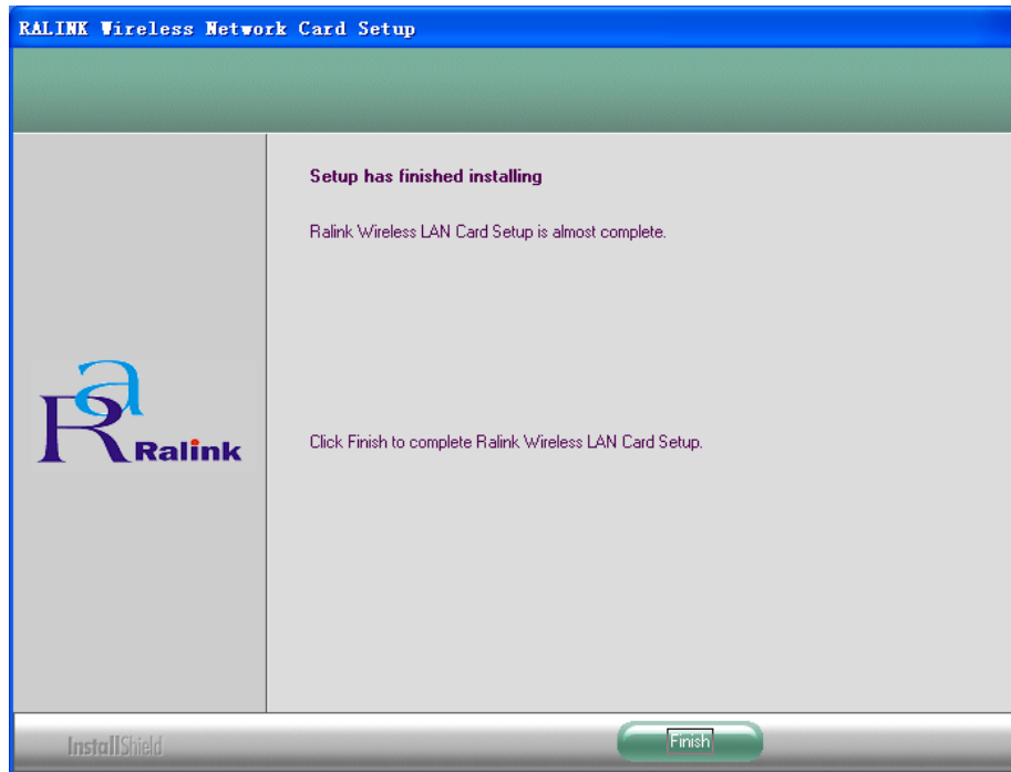
Figure 2-4 Finish installing
