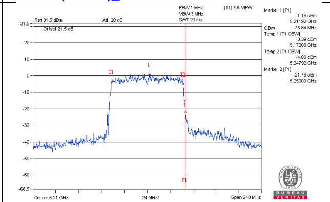
802.11ac(VHT80)_Chain1 / CH42
