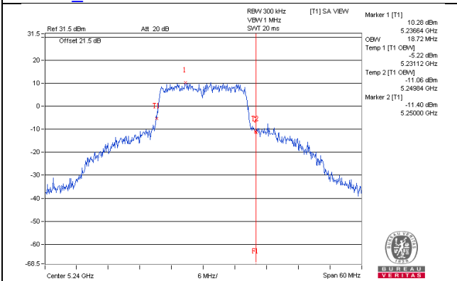
802.11ac(VHT20)_Chain0 / CH48
