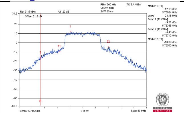
802.11ac(VHT20)_Chain1 / CH149
