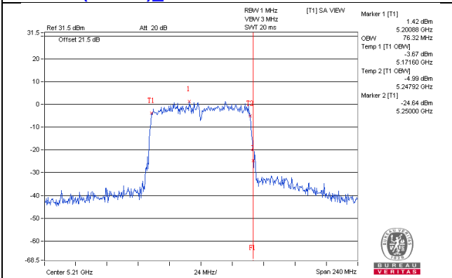
802.11ac(VHT80)_Chain0 / CH42
