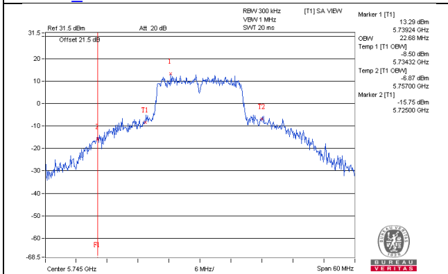
802.11ac(VHT20)_Chain0 / CH149
