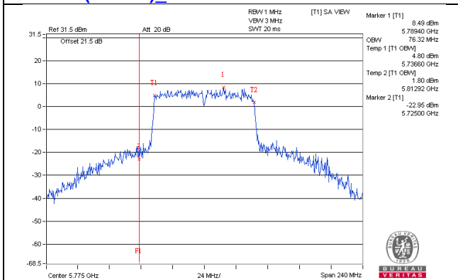
802.11ac(VHT80)_Chain0 / CH155
