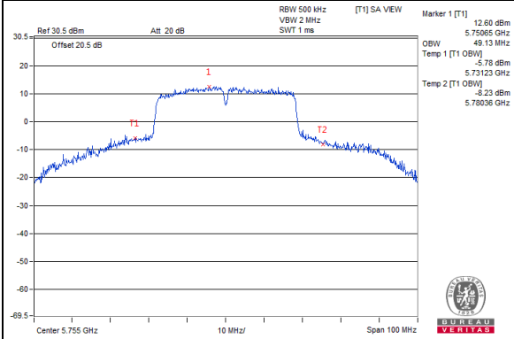
802.11n (40MHz)_Chain0 / CH151
