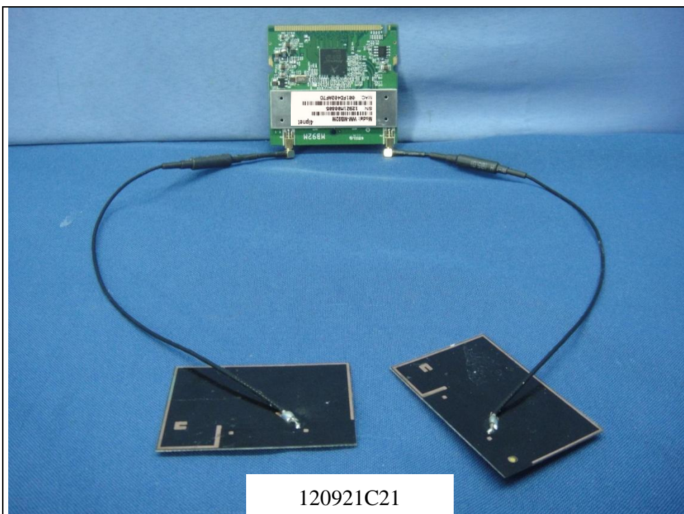
With PIFA antenna
