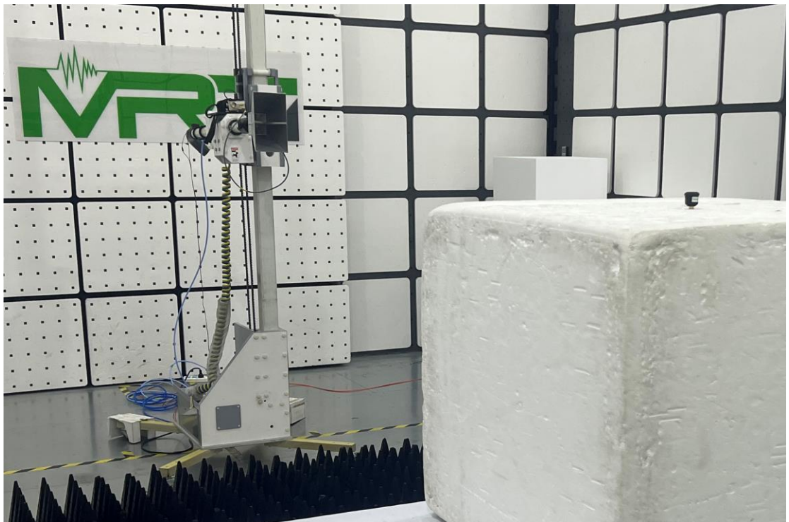
Description: Zoom for Radiated Emission Test Setup for Above 1GHz
