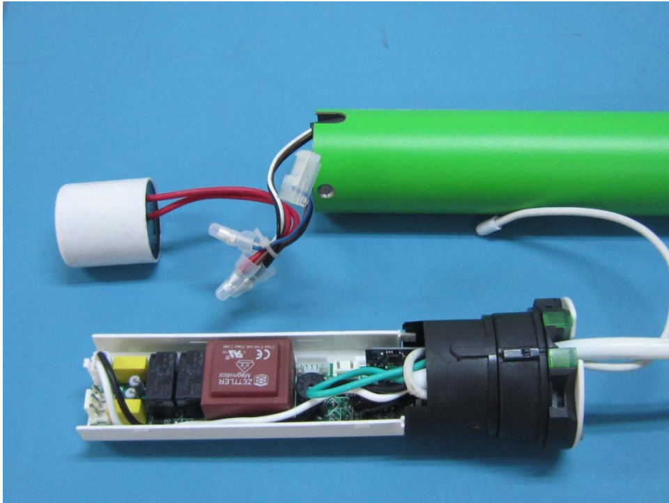
Model: DM45EQ/S-10/21
