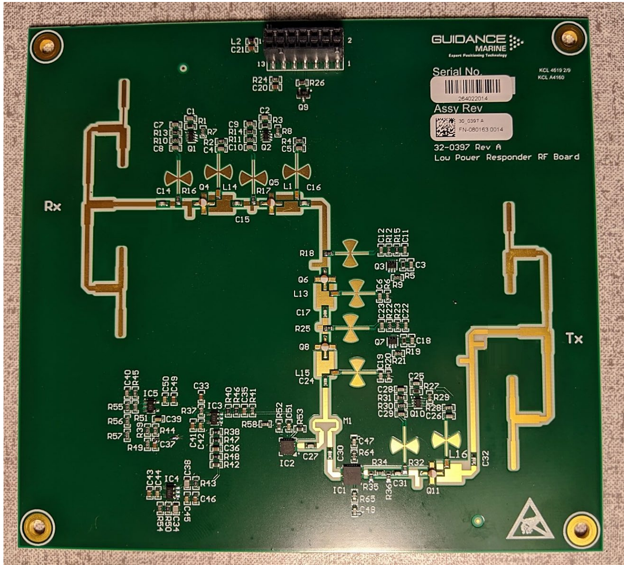
Antenna PCB, Back
