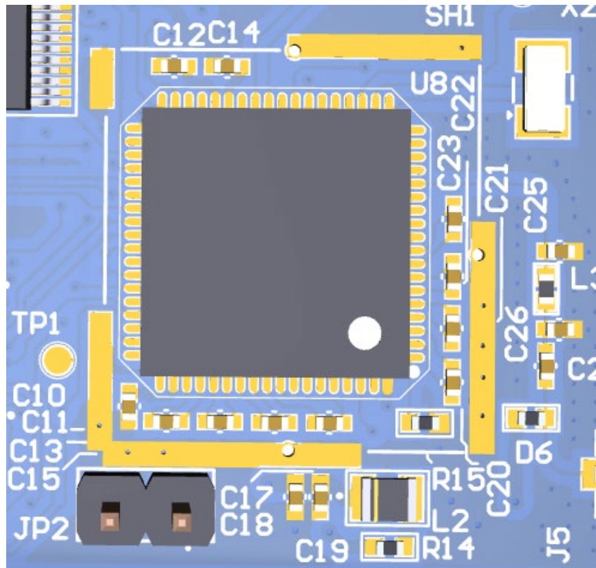
Circuitry under the shield circled in orange on A4010 Top View.
