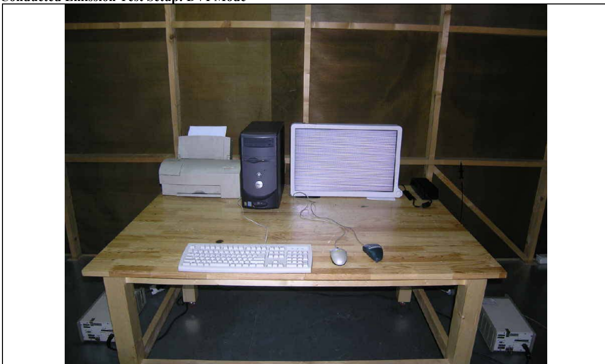
Figure 1 Conducted Emission Test Setup: DVI Mode
