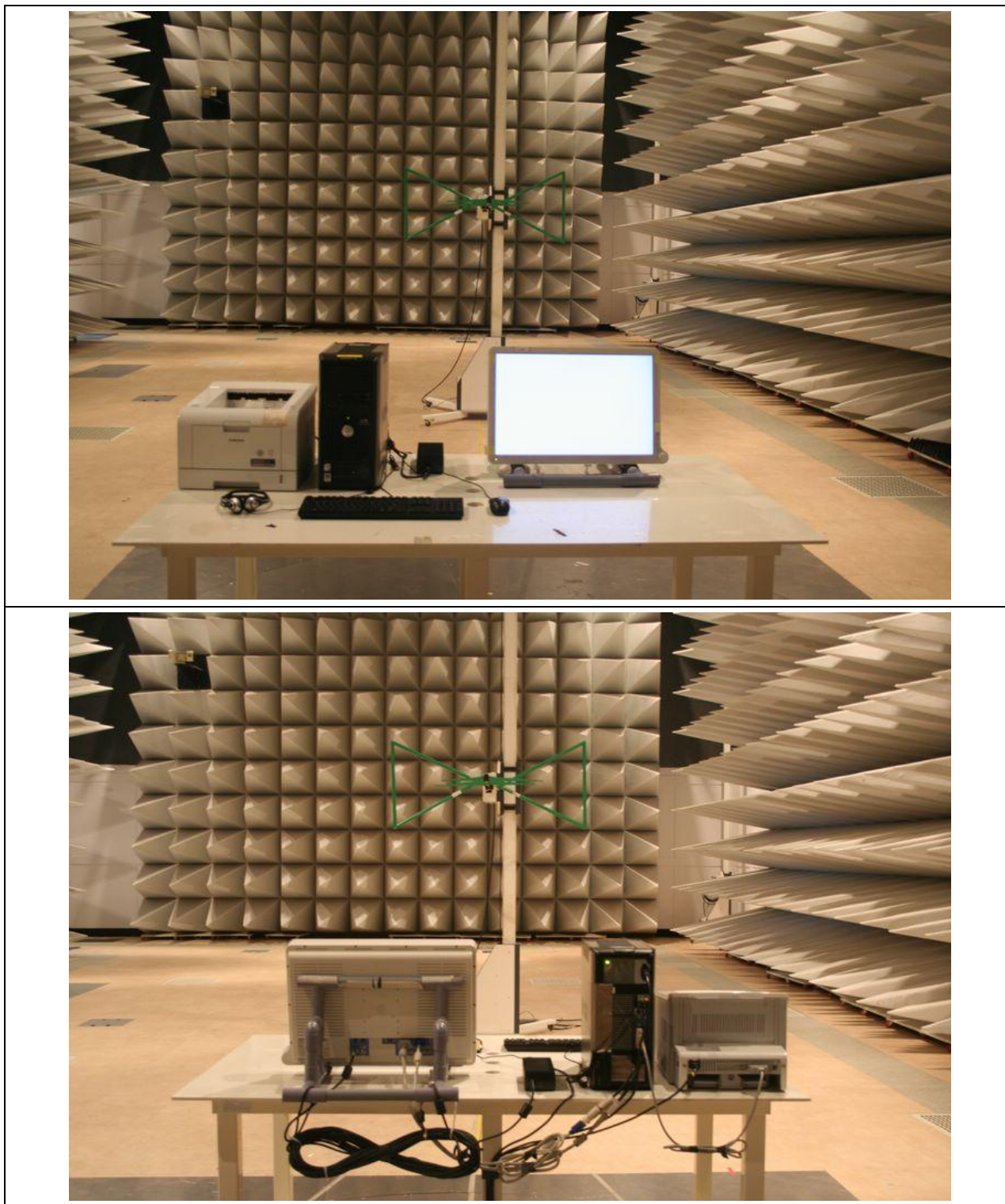
Figure 3. Photo of Radiated emission test setup for DVI Mode:
