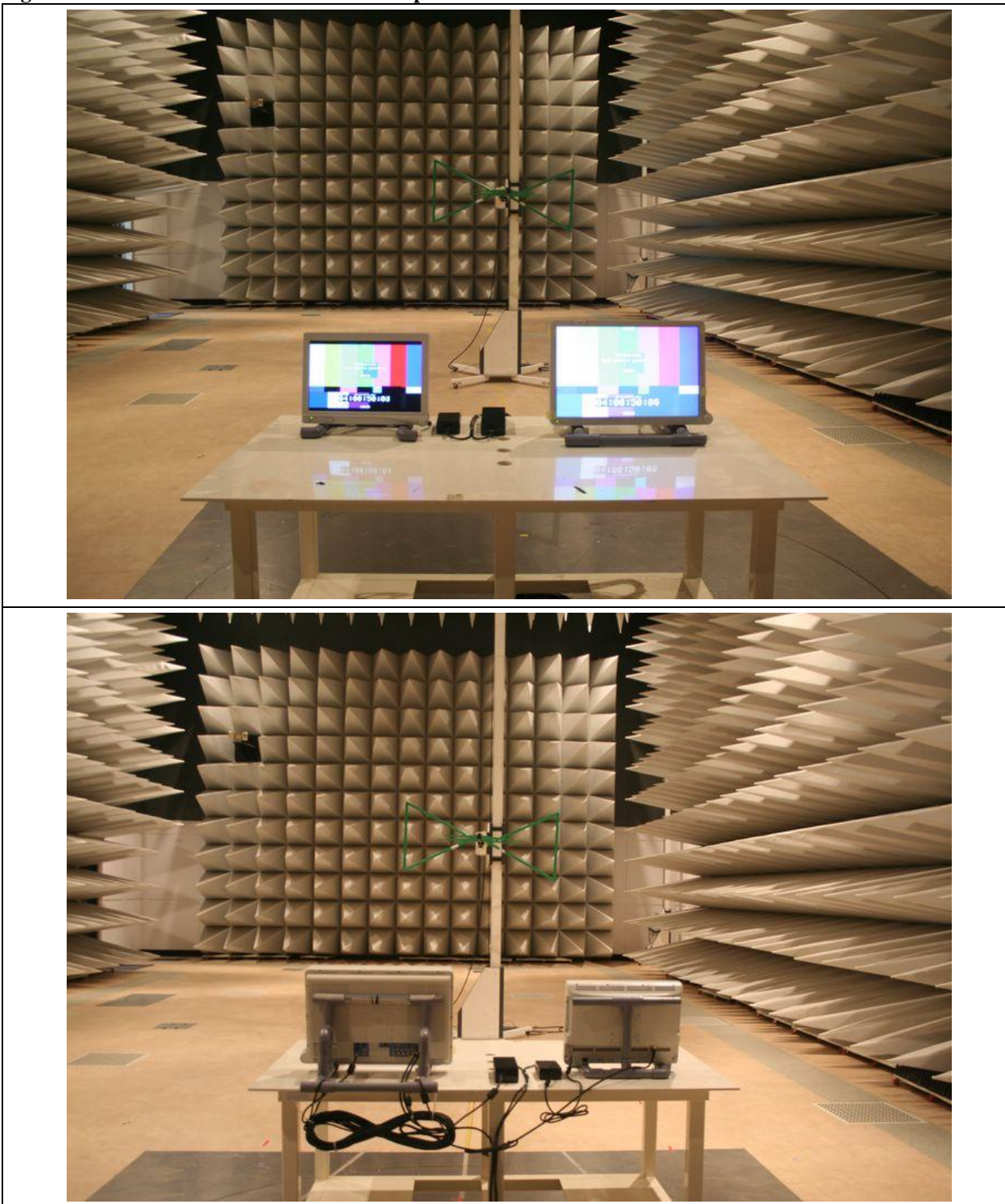
Figure 4. Photo of Radiated emission test setup for SDI In/Out Mode
