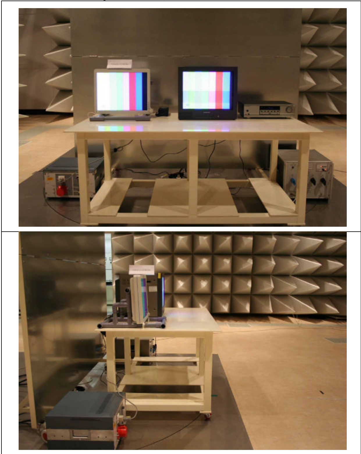
Figure 2 Conducted Emission Test Setup: S-Video Mode (LCD Panel: TX54D32VC0CAB)
