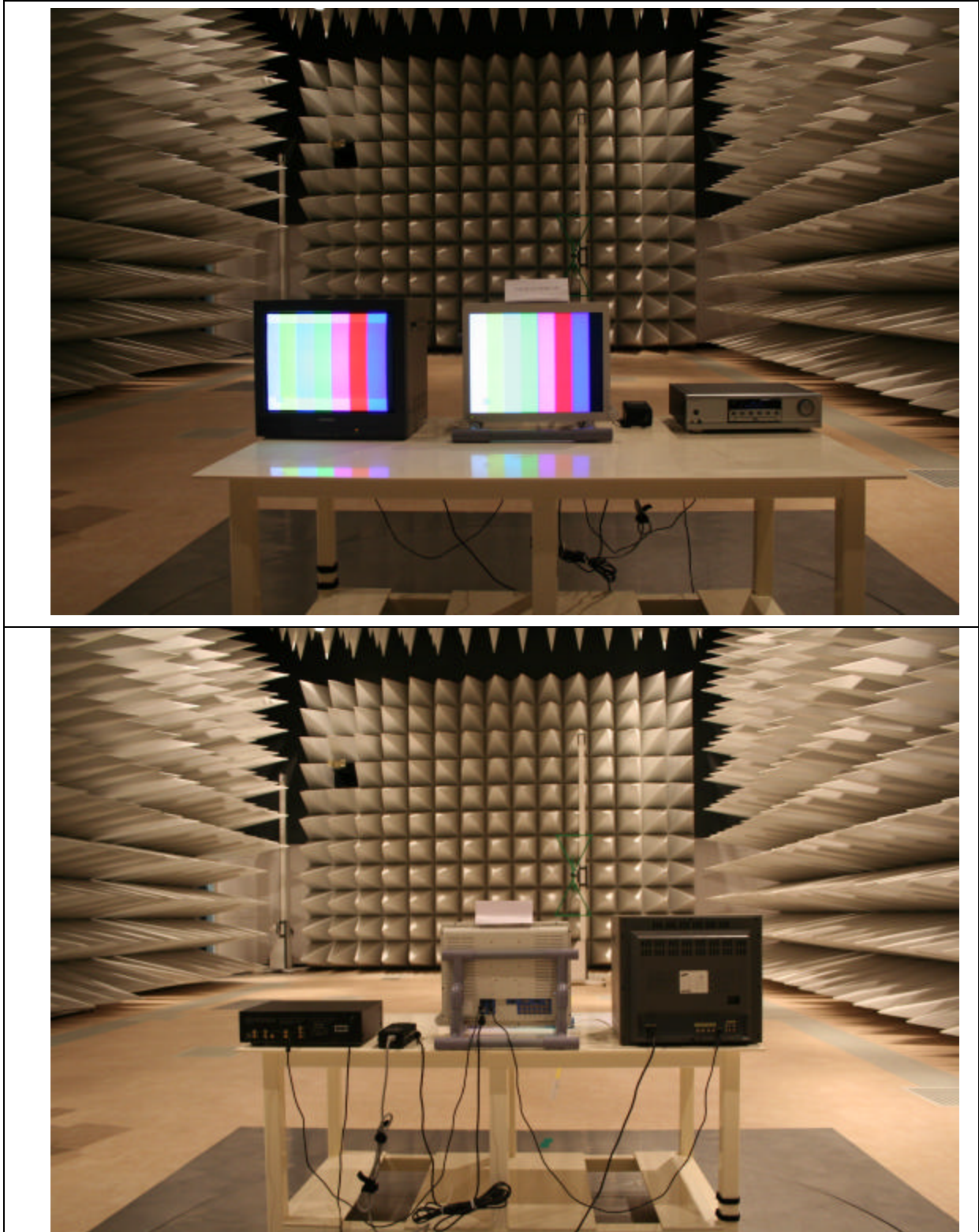
Figure 6 Photo of Radiated emission test setup: S-Video Mode (LCD Panel: TX54D32VC0CAB)
