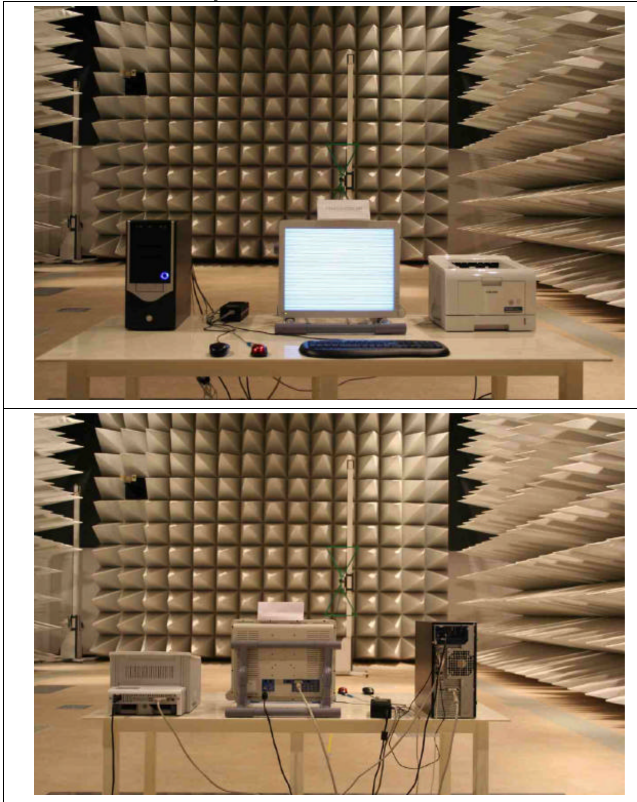
Figure 5 Photo of Radiated emission test setup: DVI Mode (LCD Panel: TX54D32VC0CAB)
