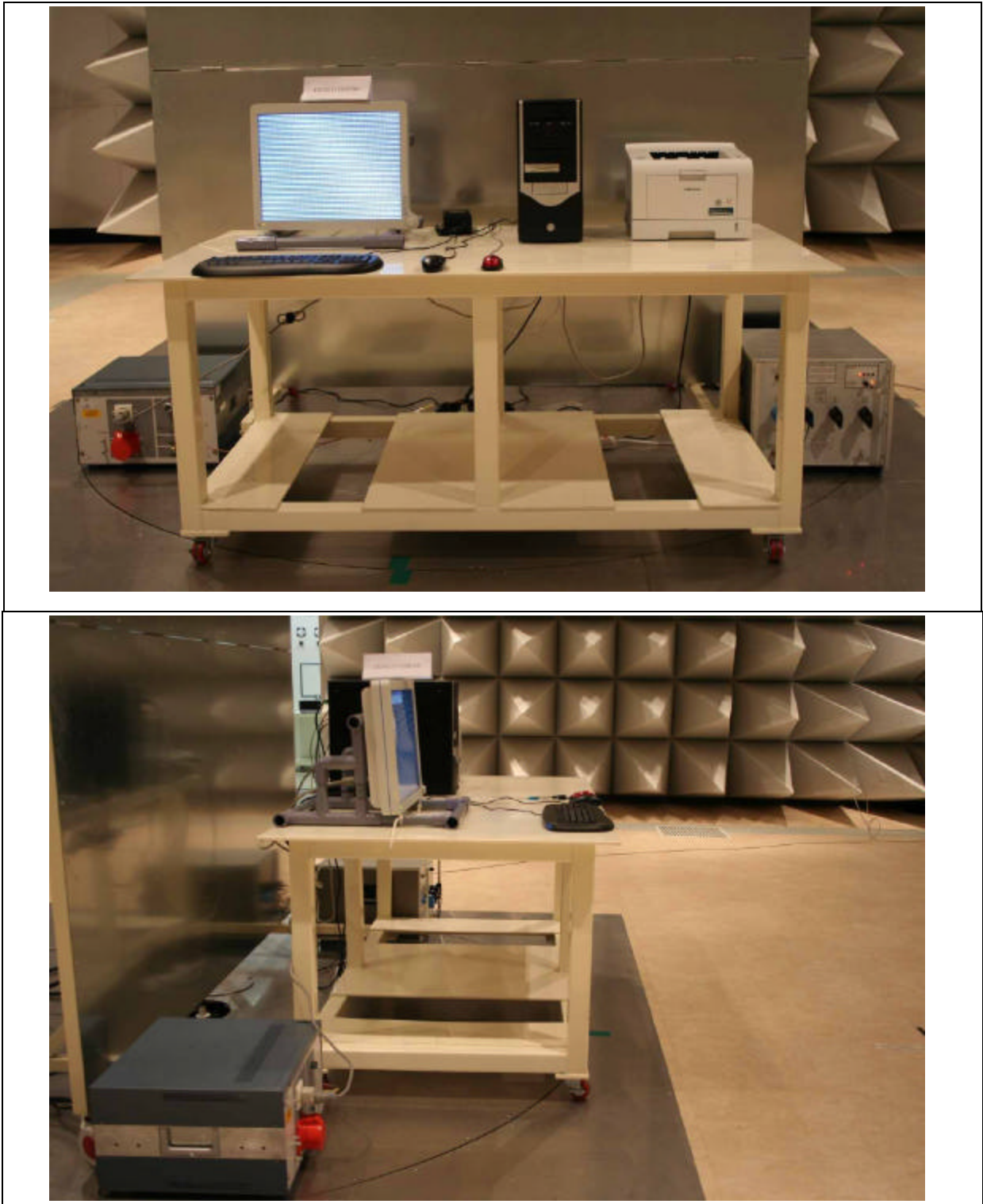
Figure 1 Conducted Emission Test Setup: DVI Mode (LCD Panel: TX54D32VC0CAB)
