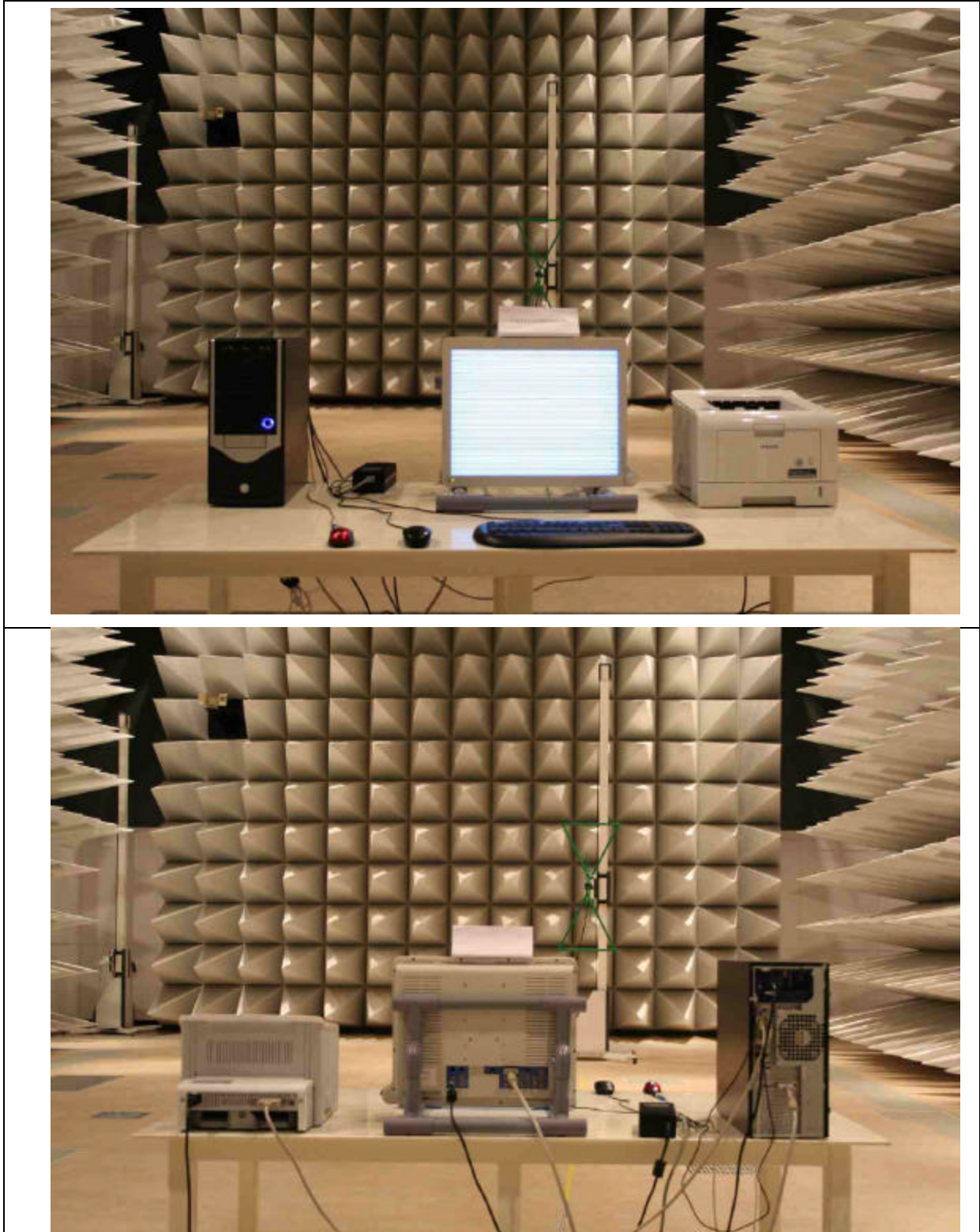
Figure 7 Photo of Radiated emission test setup: DVI Mode (LCD Panel: TX54D32VC0CAA)
