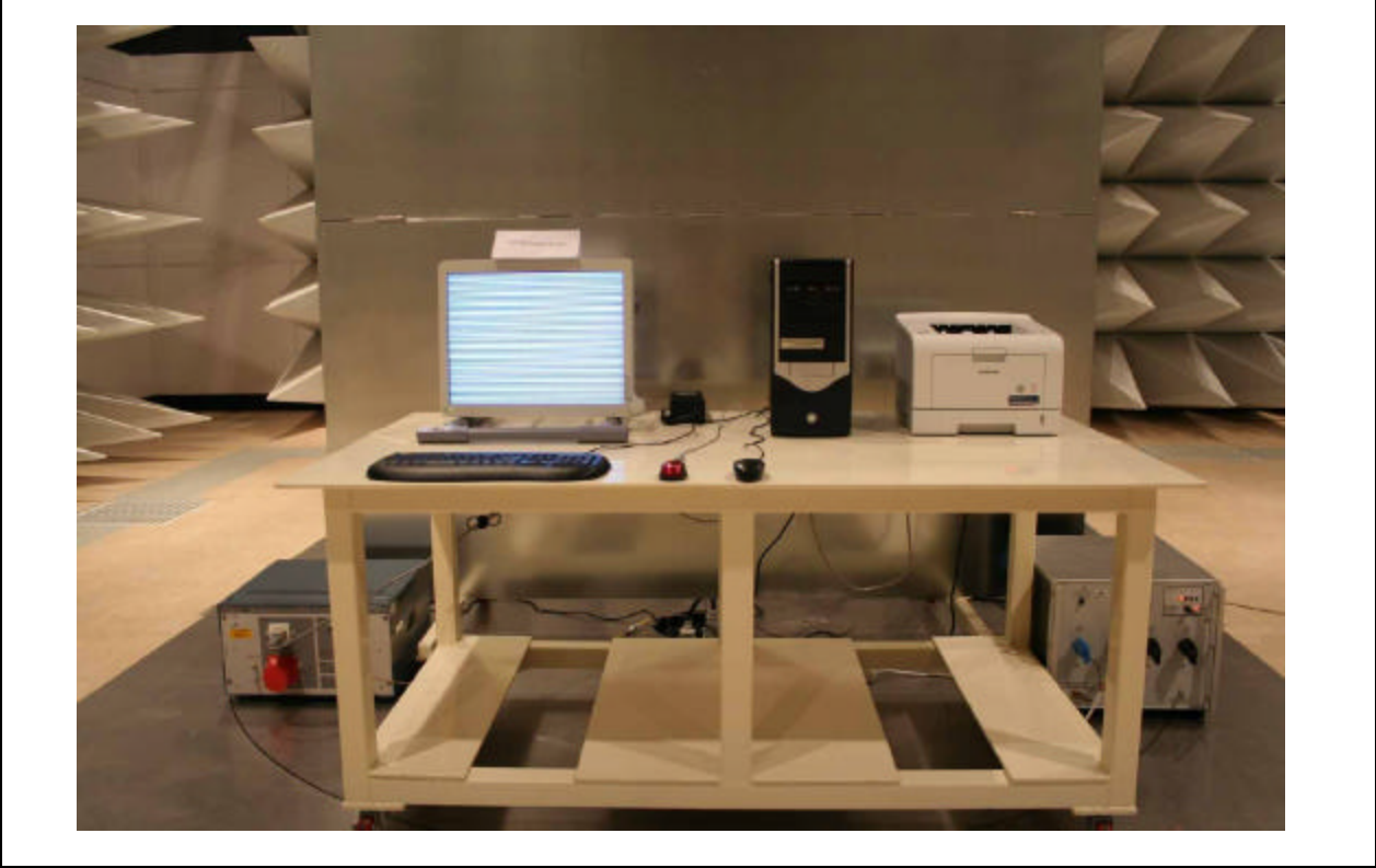
Figure 3 Conducted Emission Test Setup: DVI Mode (LCD Panel: TX54D32VC0CAA)
