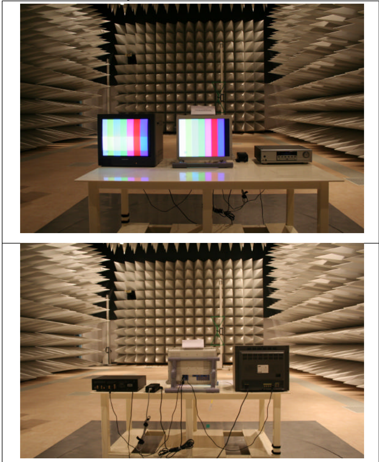
Figure 8 Photo of Radiated emission test setup: S-Video Mode (LCD Panel: TX54D32VC0CAA)
