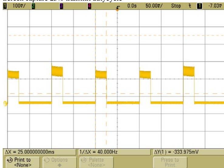
Screen capture 25% transmit dutycycle
