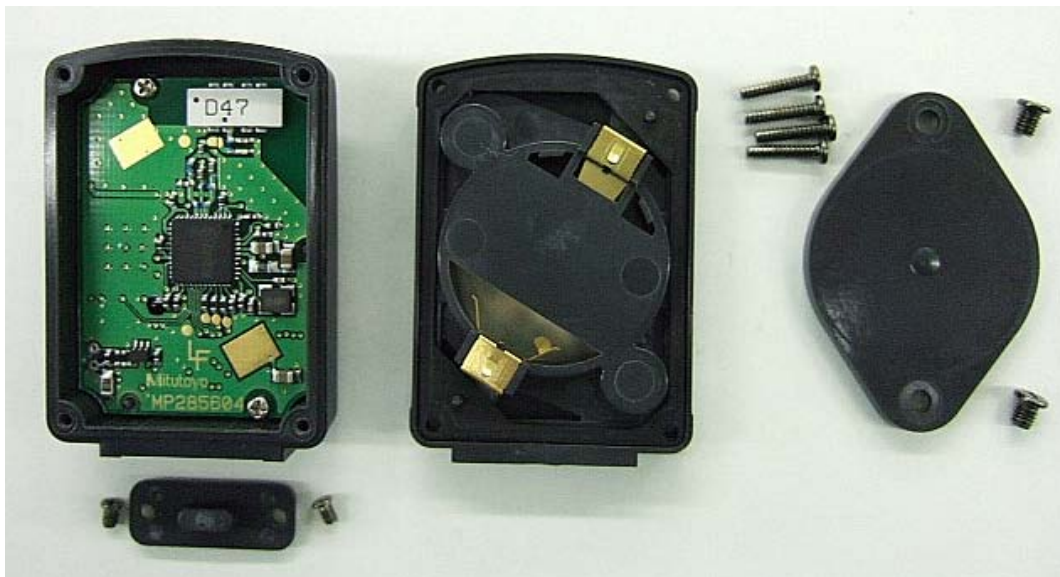
U-WAVE-T/ 02AZD880C Board with case Internal Photos1
