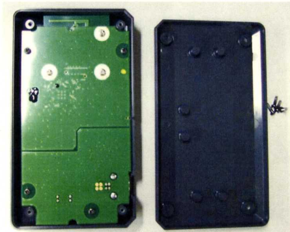
U-WAVE-R/ 02AZD810D Boards with case Internal Photo1
