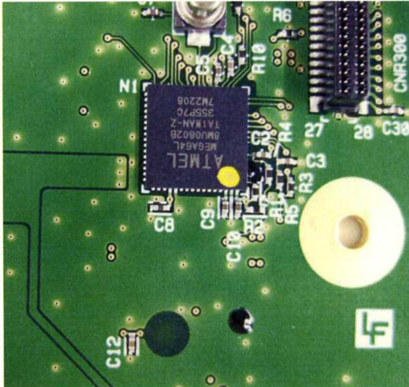
U-WAVE-R/ 02AZD810D CPU Board with putting on plastic material Internal Photo (3 of 4) Surface/ Detail of plastic material part
