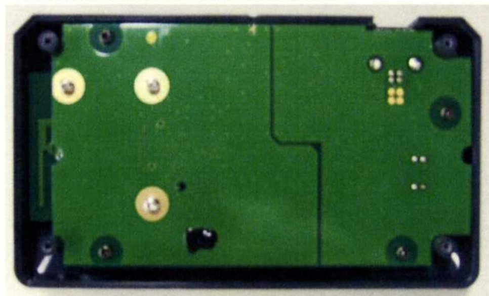
U-WAVE-R/ 02AZD810D Boards with case Internal Photo2
