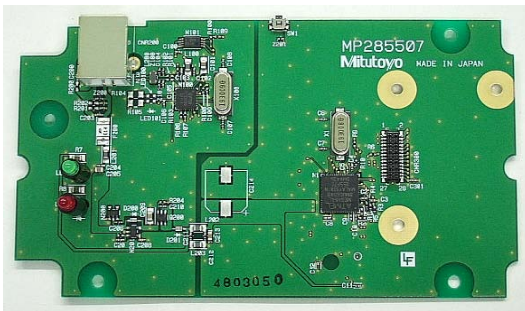
U-WAVE-R/ 02AZD810C CPU Board without plastic material Internal Photo (4 of 4) Surface
