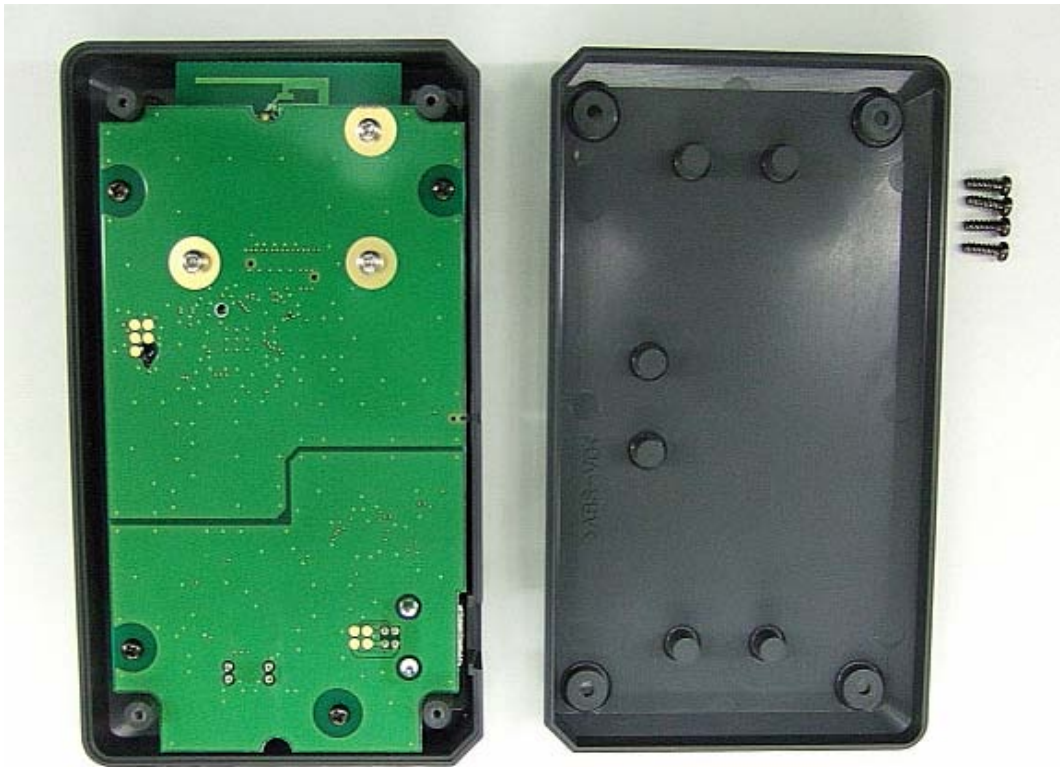
U-WAVE-R/ 02AZD810C Boards with case Internal Photo1
