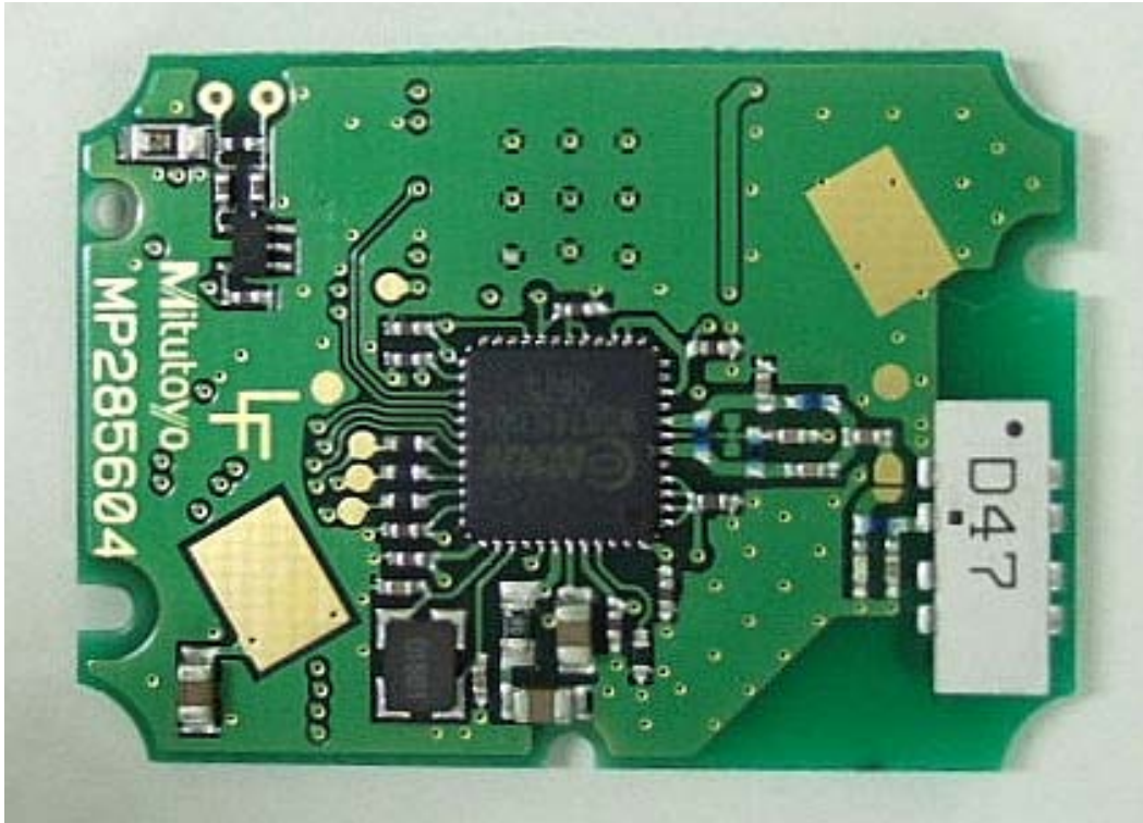
U-WAVE-T/ 02AZD730C without plastic material Internal Photos Surface
