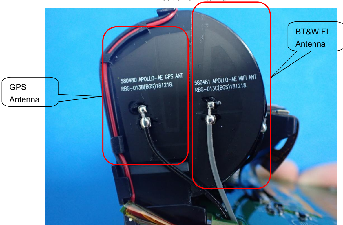
Position of Antenna
