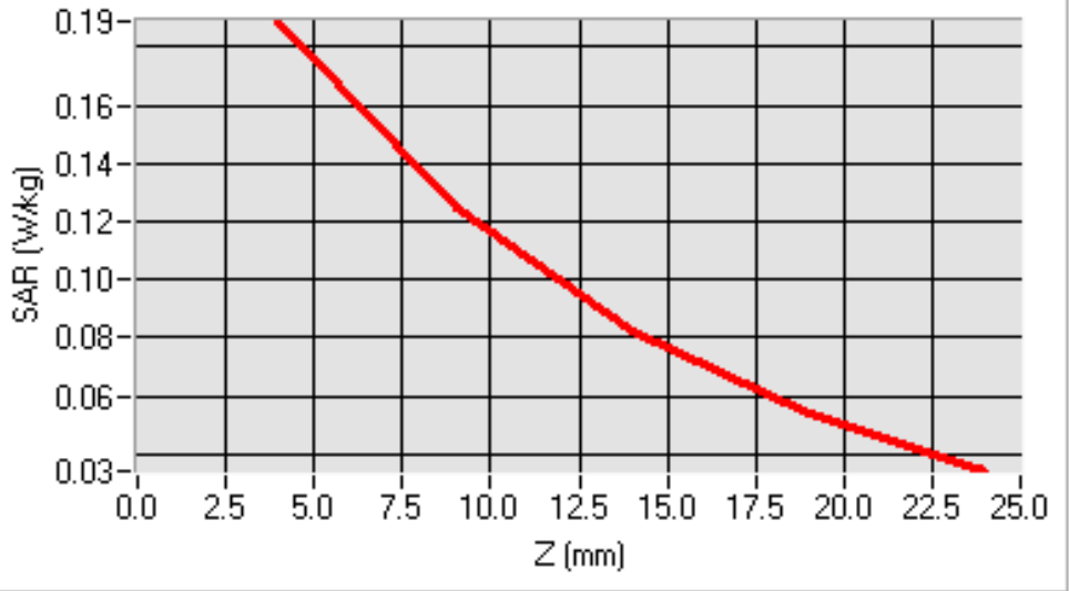
SAR, Z Axis Scan (X = 1, Y = -24)
