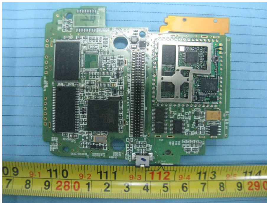
EUT – T700-MB Board Bottom Shielding off View
