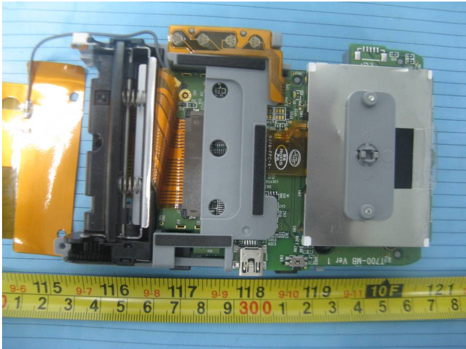
EUT – Display Cover off View
