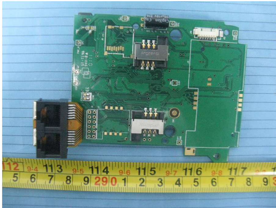
EUT – T700-ITF Board Bottom View
