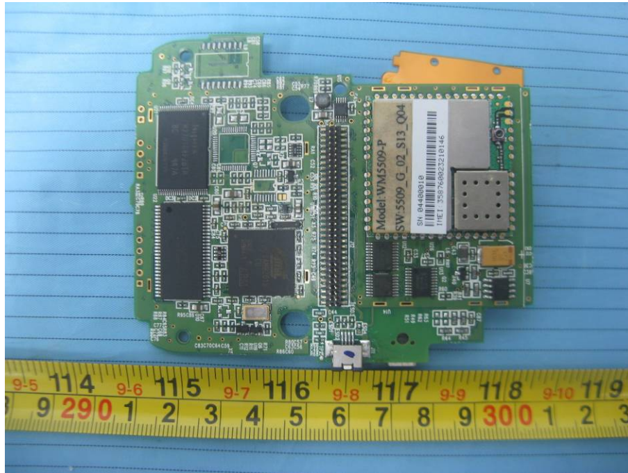
EUT – T700-MB Board Bottom View
