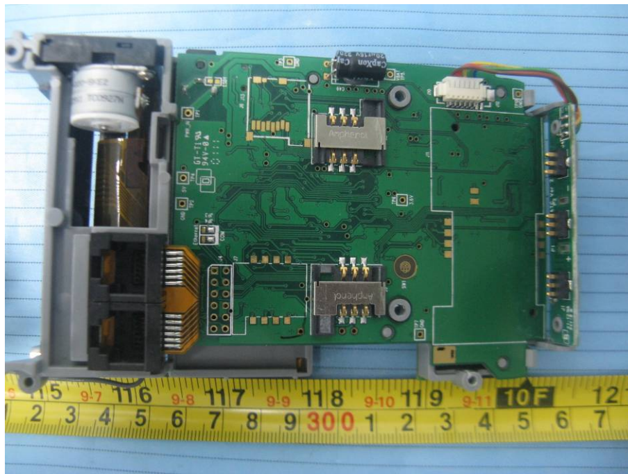
EUT – T700-ITF Board Bottom with Printer View
