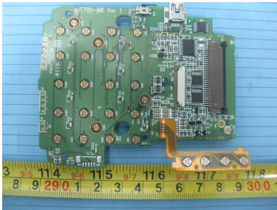
EUT – T700-MB Board Top View
