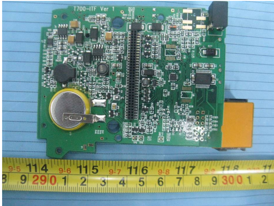
EUT – T700-ITF Board Top View
