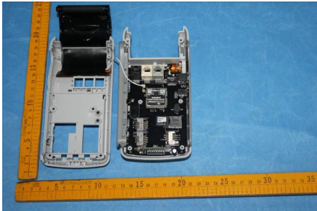
Figure 8 The EUT-Inside View
