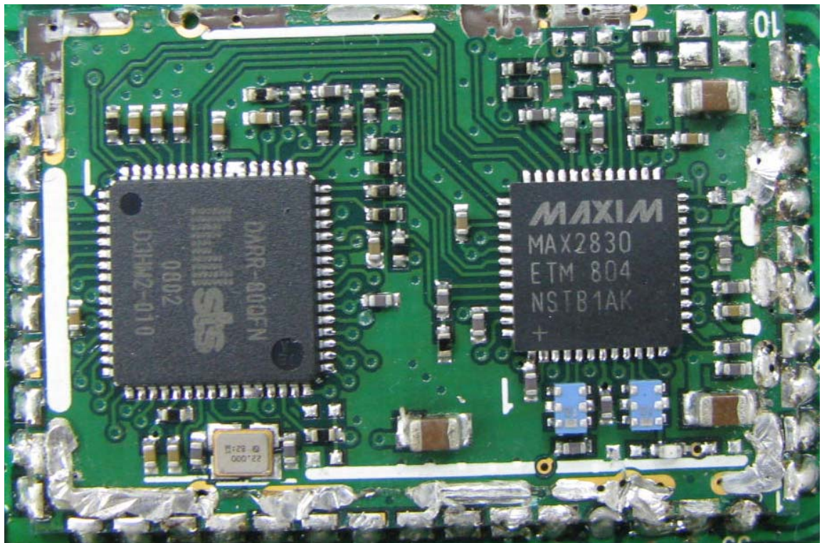
Figure 9-RF Module 1
