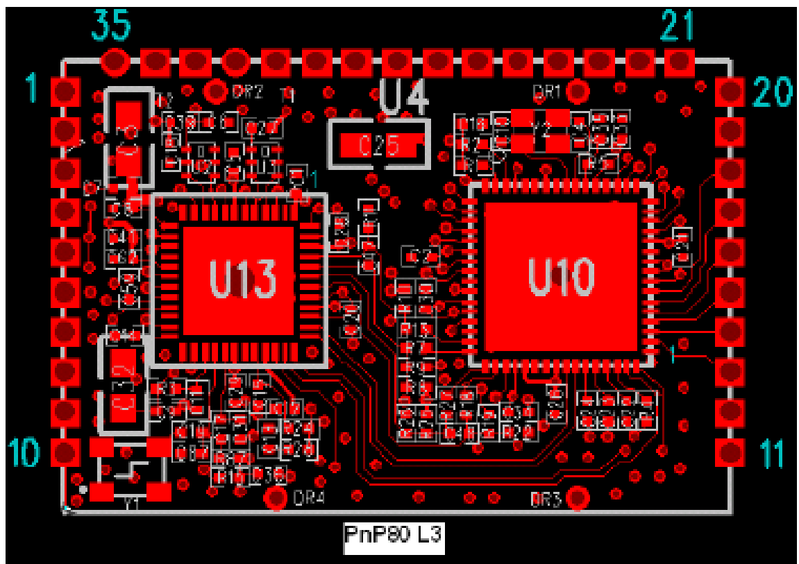
Figure 10-RF Module lay out
