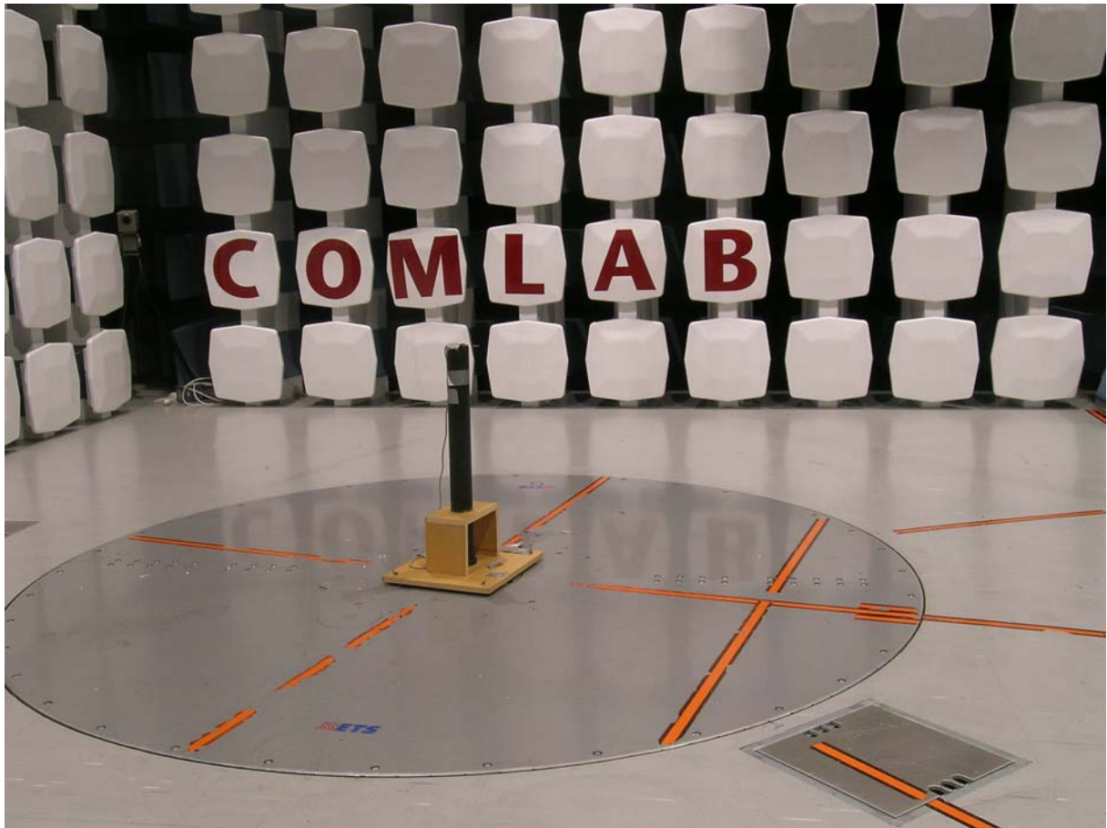
USB – Radiated measurements
