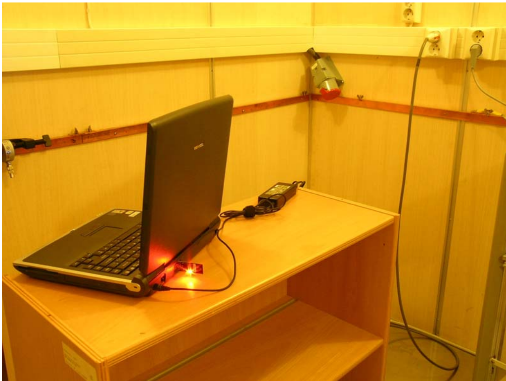
USB – Power line conducted emission
