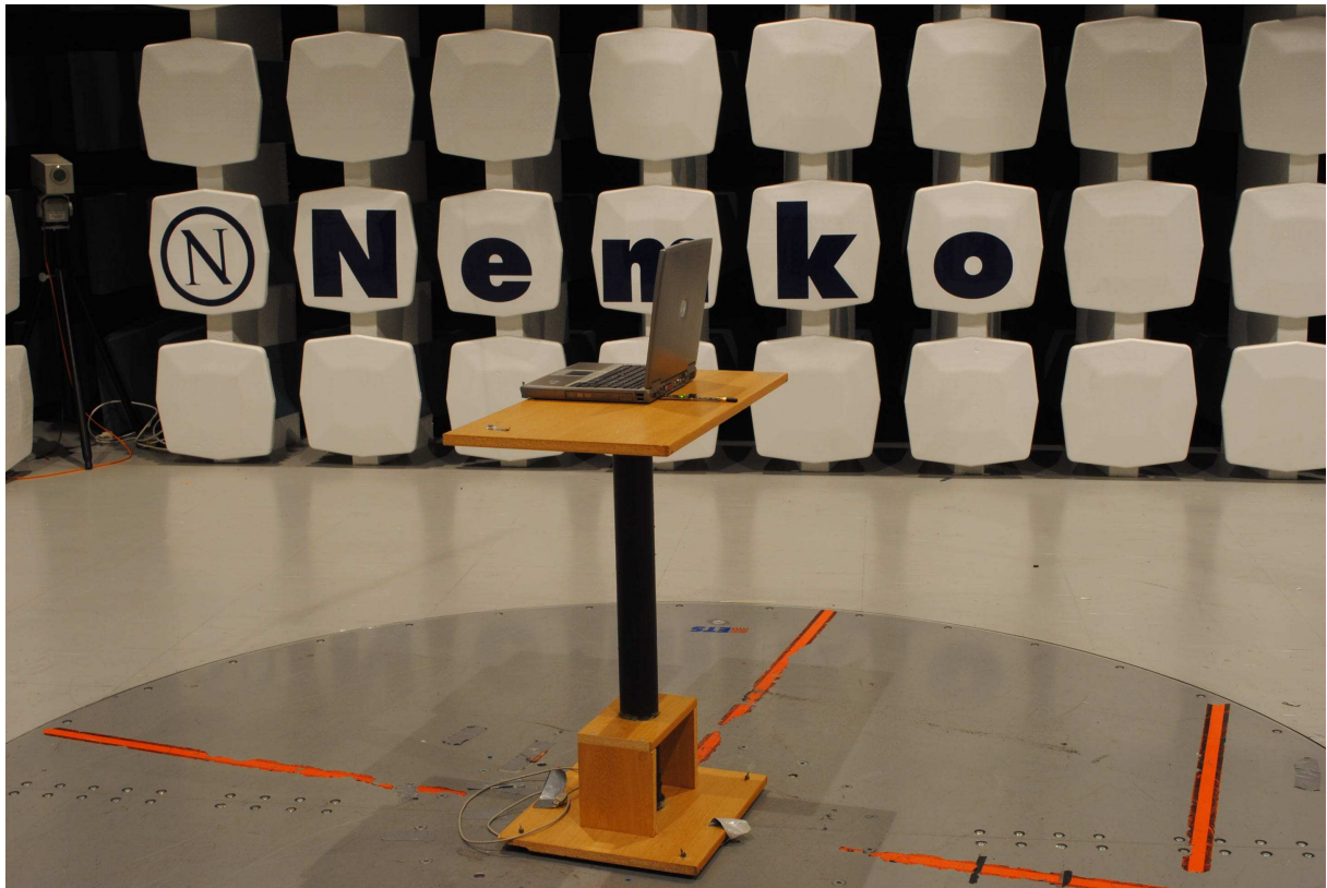
USB – Radiated measurements
