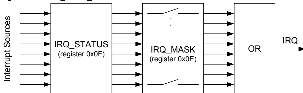
Figure 4-18. IRQ_MASK_MODE = 1
