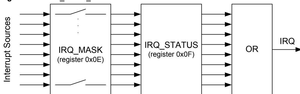
Figure 4-17. IRQ_MASK_MODE = 0
