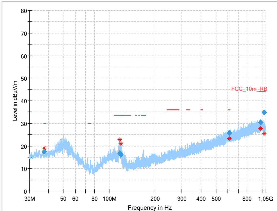
Plot 1: 30 MHz to 1 GHz, TX mode, vertical & horizontal polarization, Valid for all channels of 1 Msps
