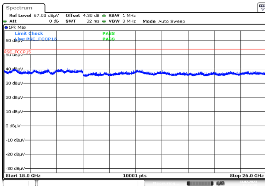
Plot 1: 18 GHz to 26 GHz, vertical & horizontal polarization
