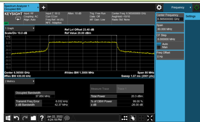
Channel 123 (6565MHz)
