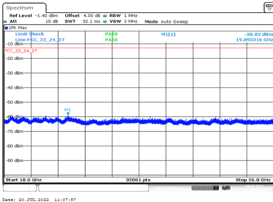
Plot 20: 256-QAM - Middle channel (18 GHz – 26 GHz)
