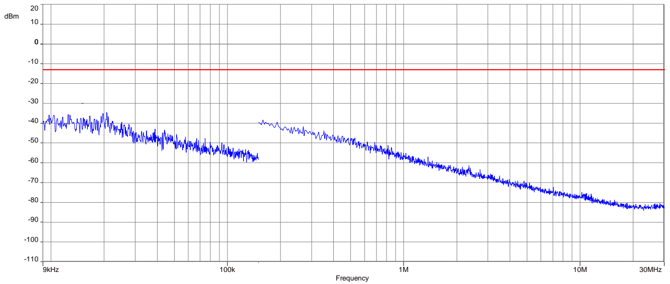
Plot 17: 256-QAM - Middle channel (9 kHz - 30 MHz)
