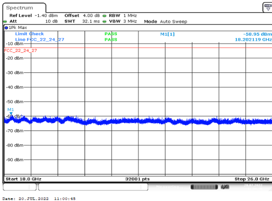
Plot 16: BPSK - Middle channel (18 GHz – 26 GHz)
