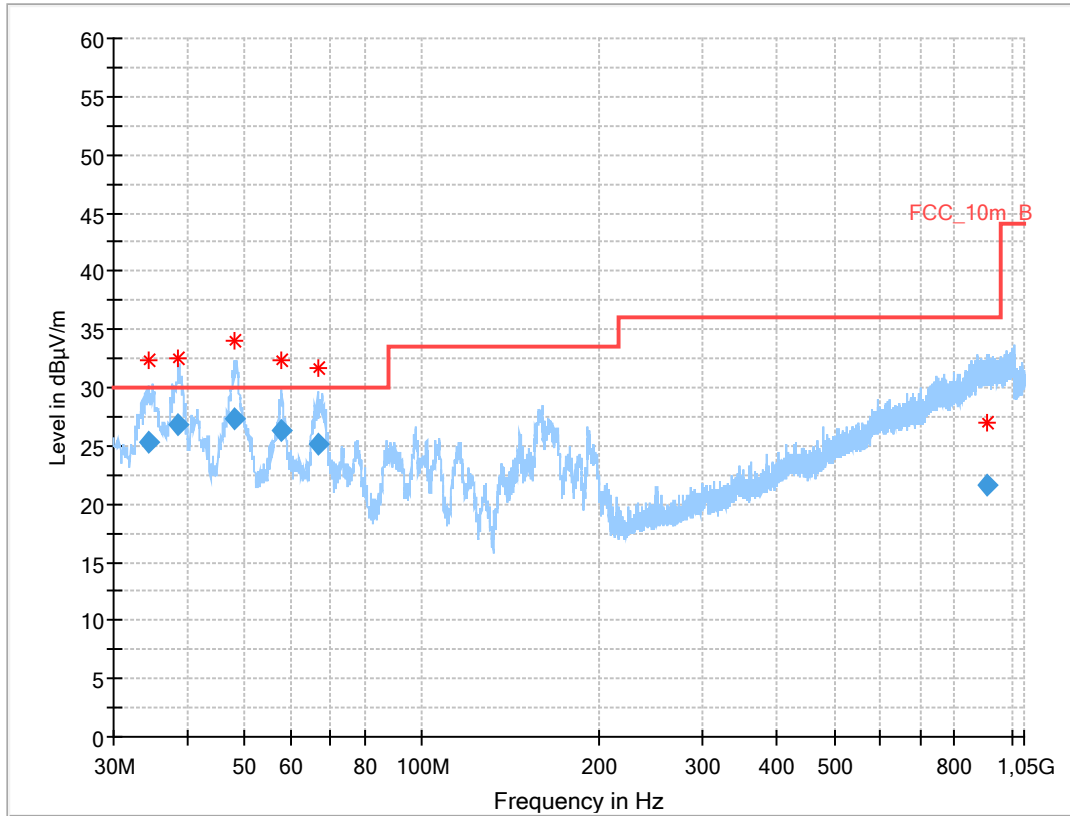
Plot 1: 30 MHz to 1 GHz; vertical & horizontal polarization; U-NII-1 & U-NII-2A; 802.11ax HE160
