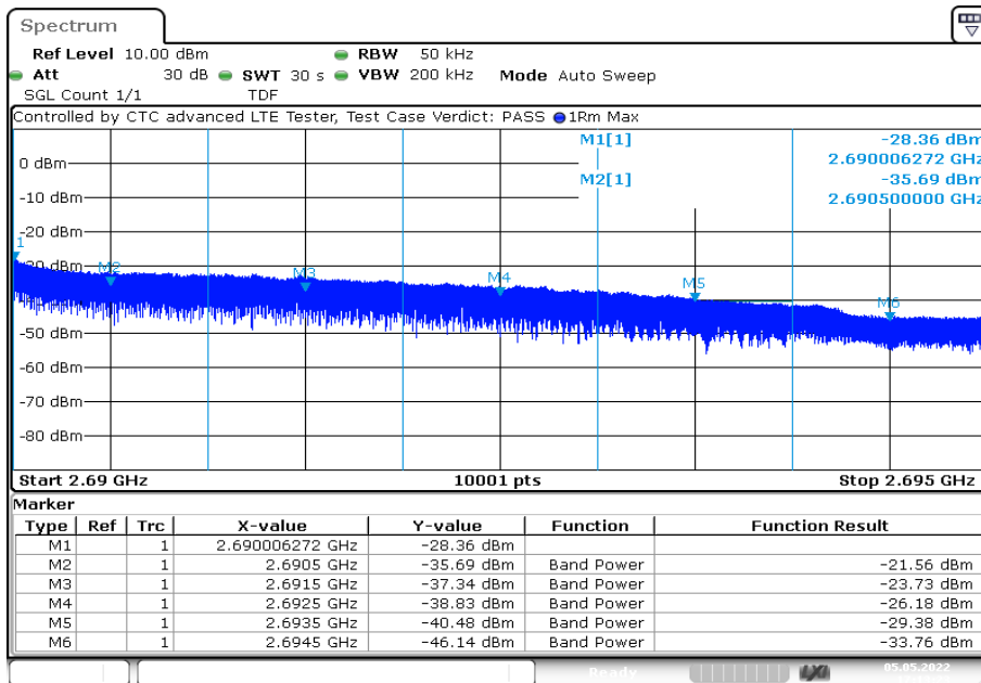
Plot 10: 5 MHz – 16-QAM - Highest channel
