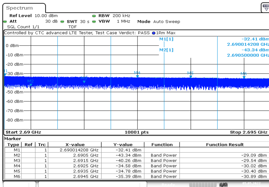
Plot 16: 20 MHz – 16-QAM - Highest channel
