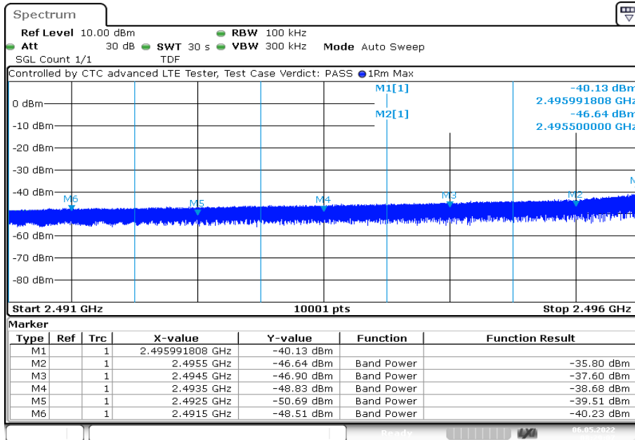
Plot 19: 10 MHz – 64-QAM - Lowest channel
