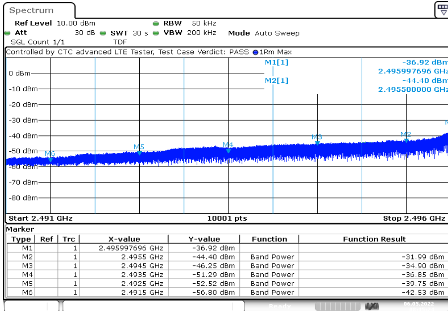
Plot 17: 5 MHz – 64-QAM - Lowest channel
