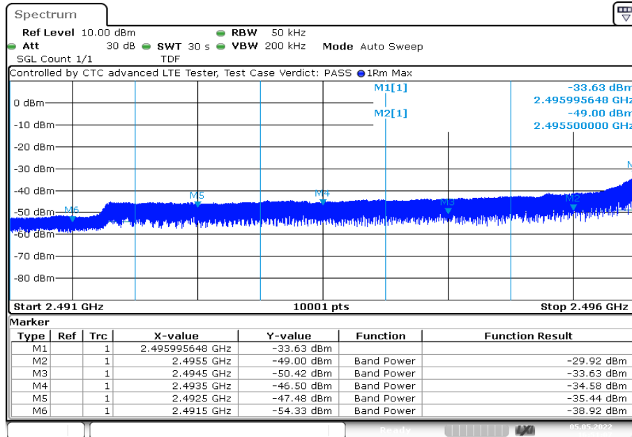
Plot 1: 5 MHz – QPSK - Lowest channel
