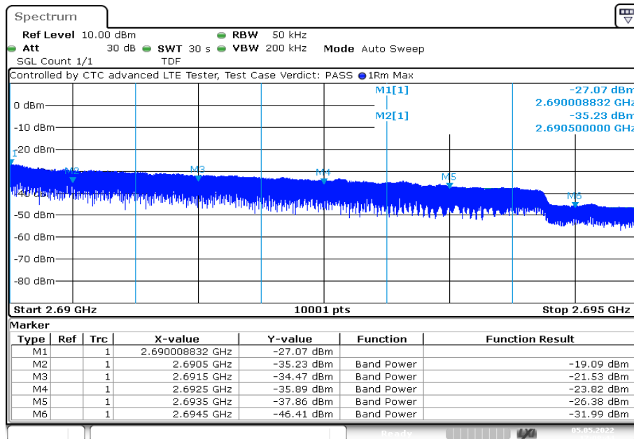
Plot 2: 5 MHz – QPSK - Highest channel
