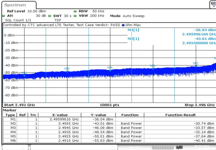
Plot 9: 5 MHz – 16-QAM - Lowest channel
