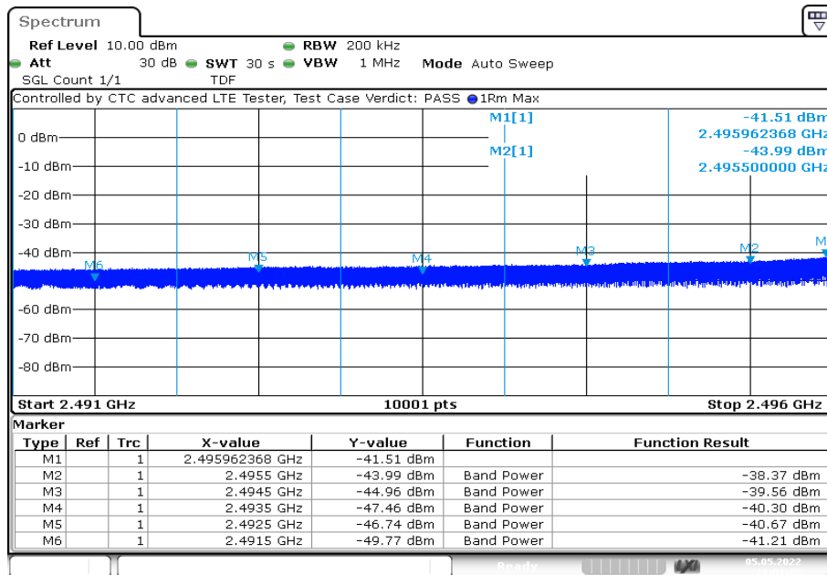
Plot 15: 20 MHz – 16-QAM - Lowest channel
