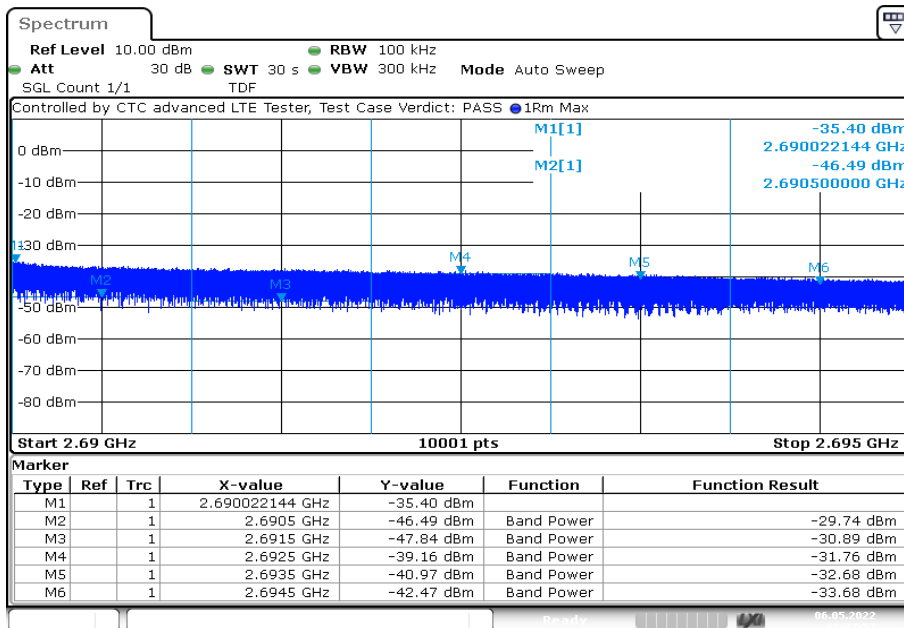
Plot 20: 10 MHz – 64-QAM - Highest channel
