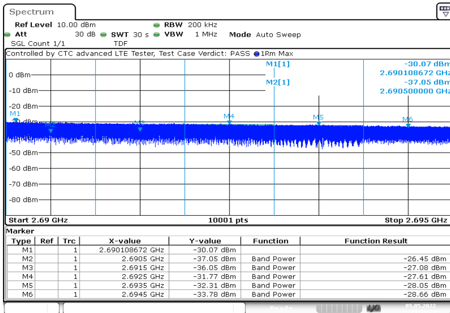
Plot 8: 20 MHz – QPSK - Highest channel
