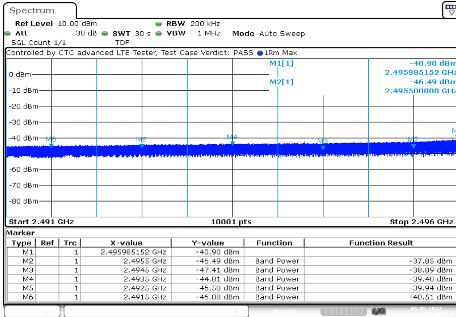
Plot 7: 20 MHz – QPSK - Lowest channel
