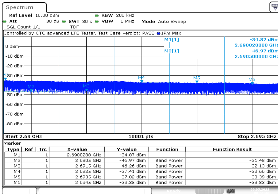
Plot 22: 15 MHz – 64-QAM - Highest channel
