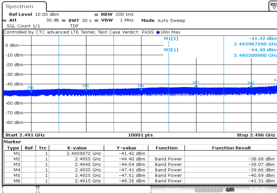
Plot 21: 15 MHz – 64-QAM - Lowest channel
