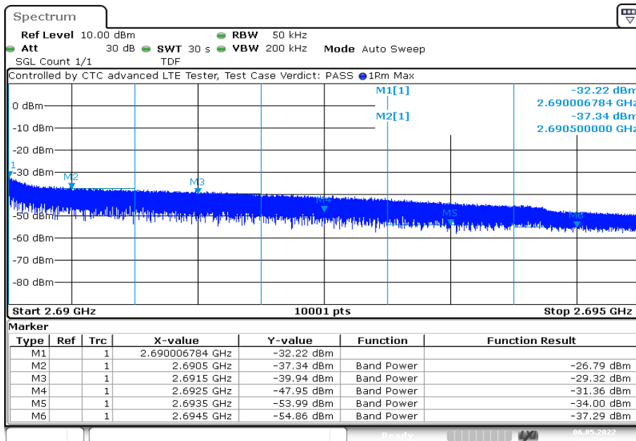
Plot 18: 5 MHz – 64-QAM - Highest channel
