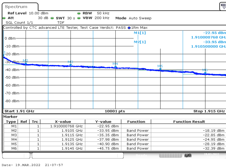
Plot 6: 5 MHz – QPSK - Highest channel
