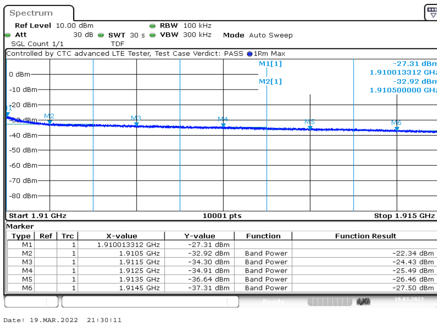
Plot 8: 10 MHz – QPSK - Highest channel
