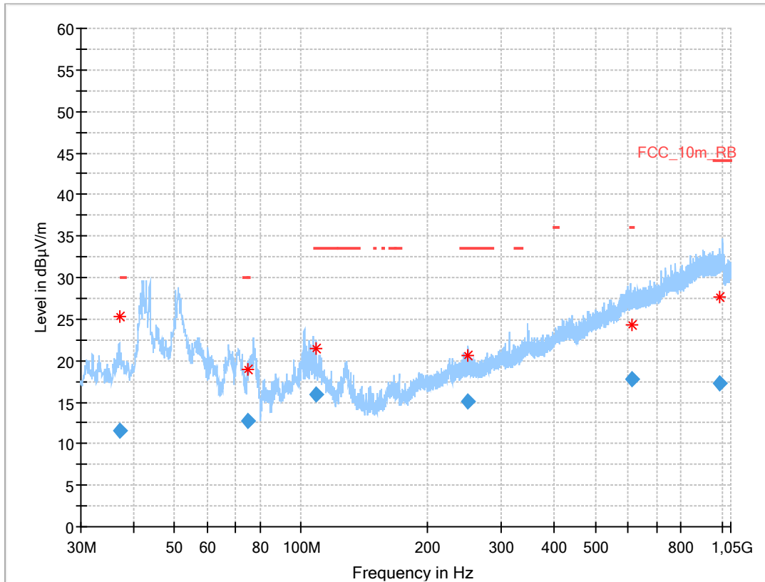
Plot 2: 30 MHz to 1 GHz, TX mode, 2440 MHz, vertical & horizontal polarization, valid for all channels of 2 Msps mode
