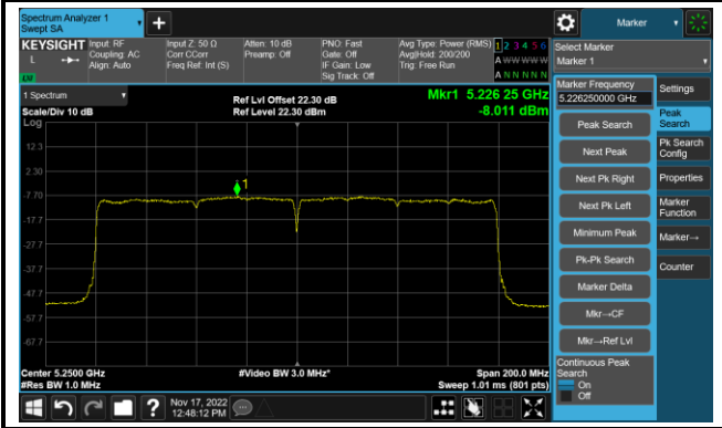
Channel 50 (5250MHz)
