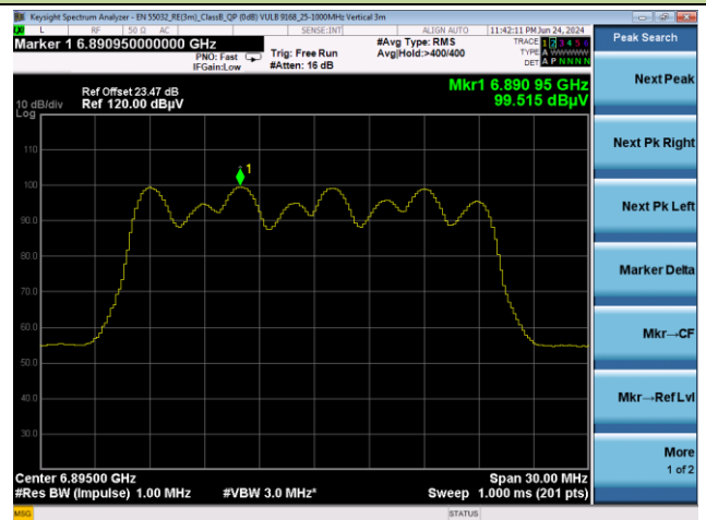
Channel 189 (6895MHz)
