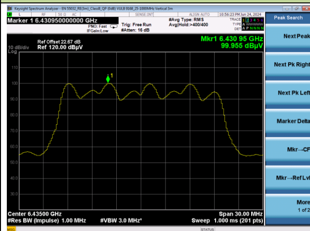
Channel 97 (6435MHz)
