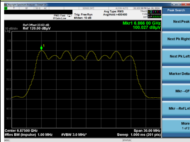
Channel 185 (6875MHz)
