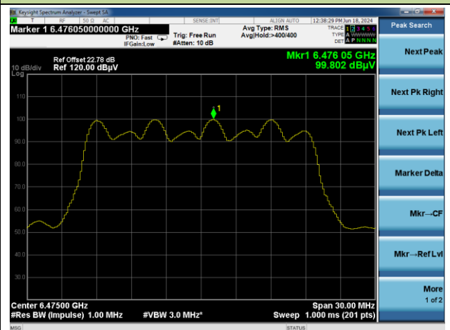
Channel 105 (6475MHz)
