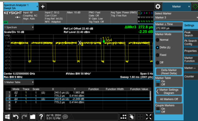
Duty Cycle (T = Transmission Duration)
