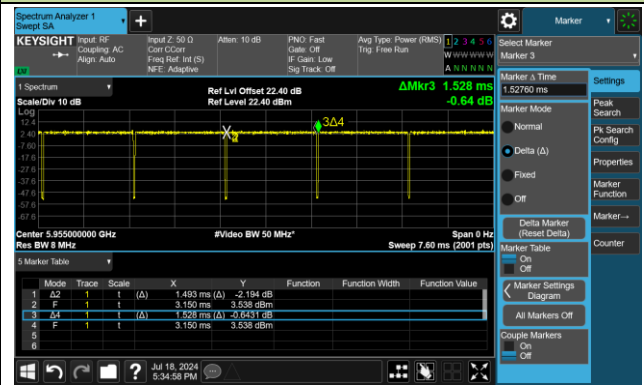
Duty Cycle (T = Transmission Duration)
