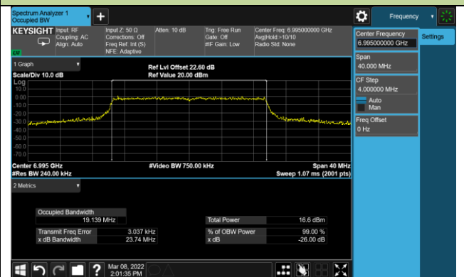
Channel 209 (6995MHz)
