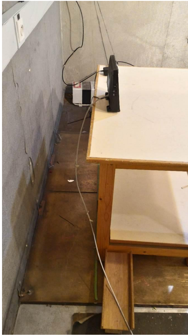
Test setup for power line conducted emissions
