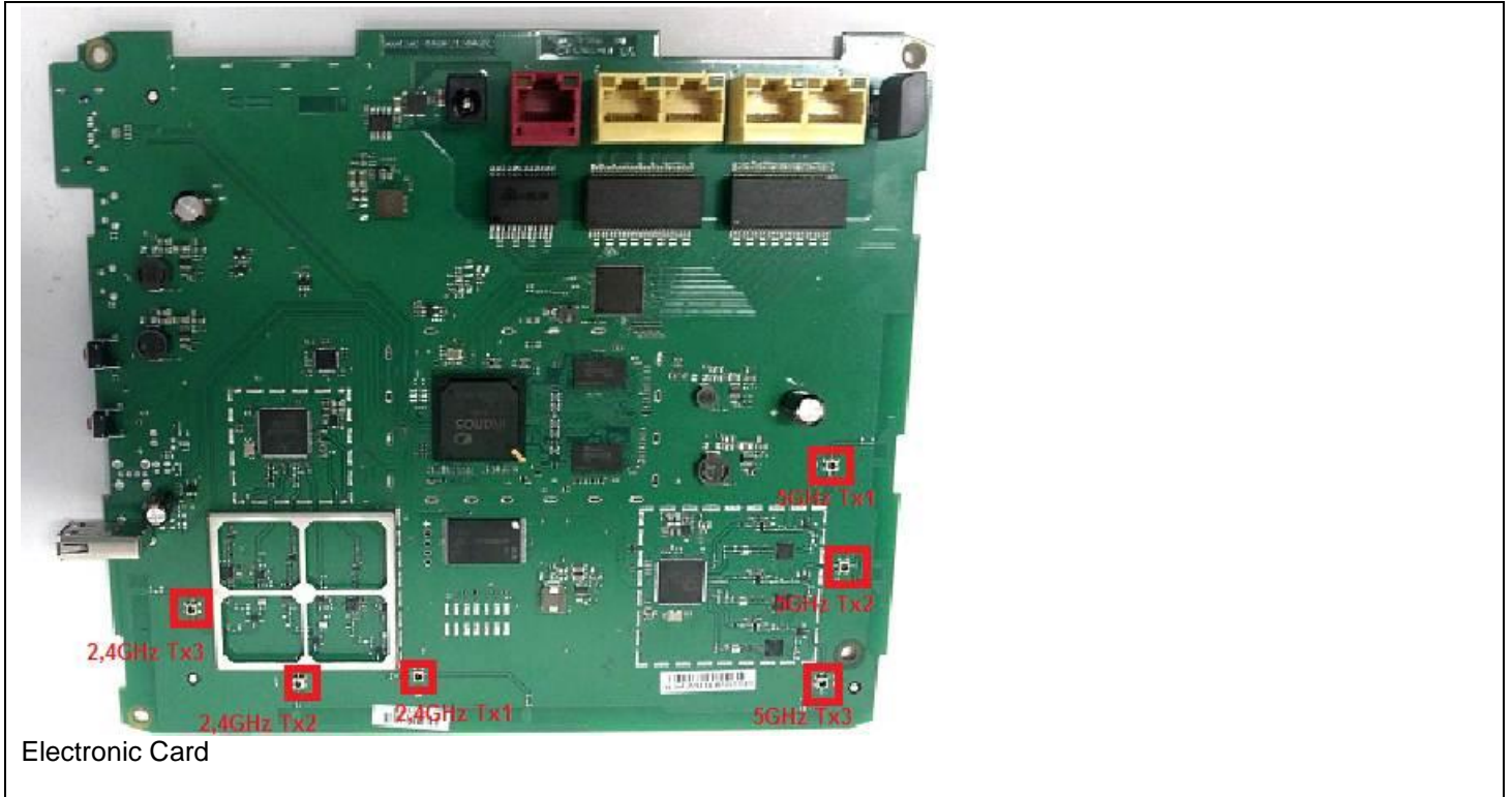
Photograph of EUT
