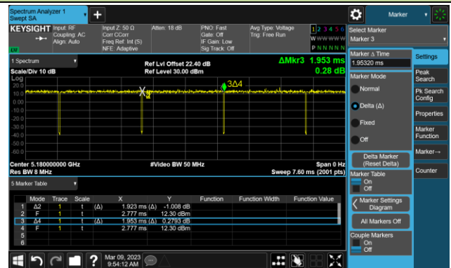
802.11ax-HE80 (T = 412.8µs)
