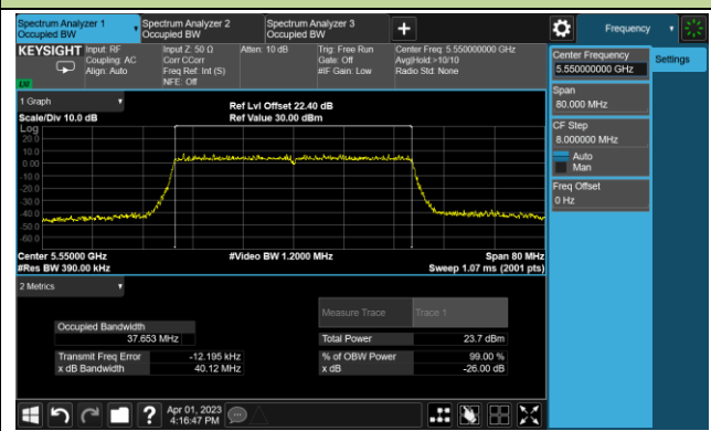
Channel 110 (5550MHz)
