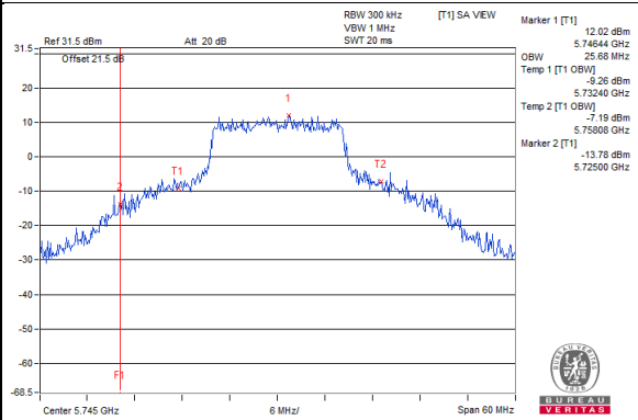
802.11ac(VHT20)_Chain0 / CH149
