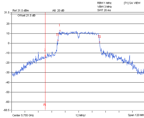
802.11ac(VHT40)_Chain1 / CH151
