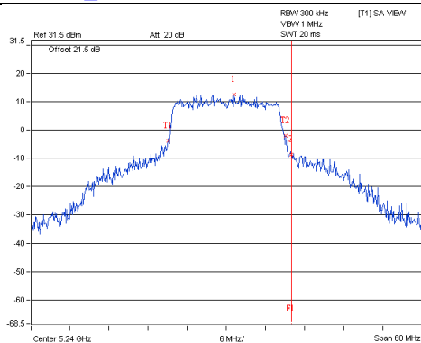
802.11ac(VHT20)_Chain0 / CH48
