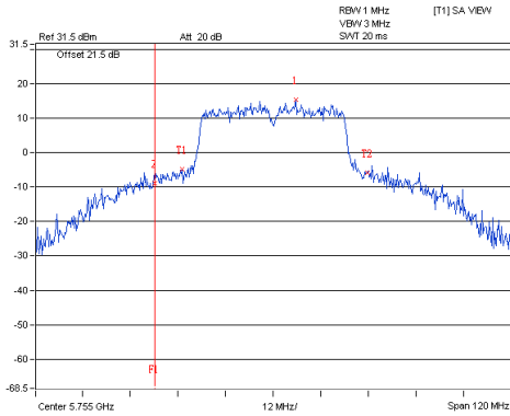
802.11ac(VHT40)_Chain2 / CH151
