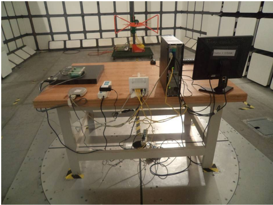
Spurious Radiated Emissions – Rear View (30 MHz - 1 GHz)
