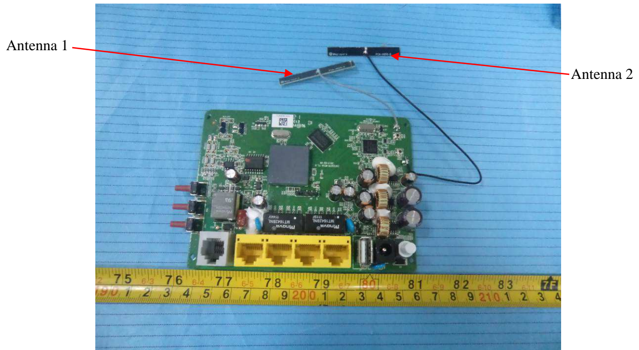
EUT – Main Board Top View 1
