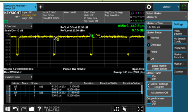
802.11ax-HE80 (T = 412.0µs)
