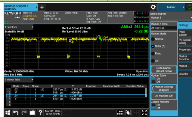
802.11ax-HE160 (T = 235.7µs)
