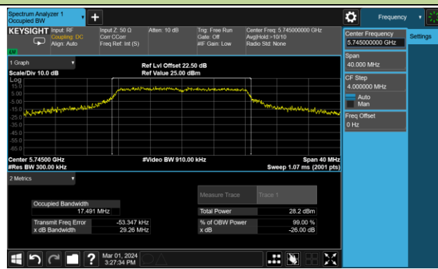
Channel 149 (5745MHz)
