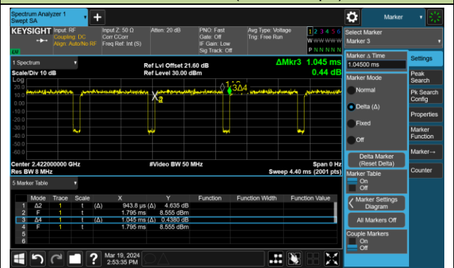
802.11n-HT40 (T = 943.8µs)
