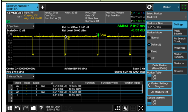
802.11n-HT20 (T = 1.918ms)
