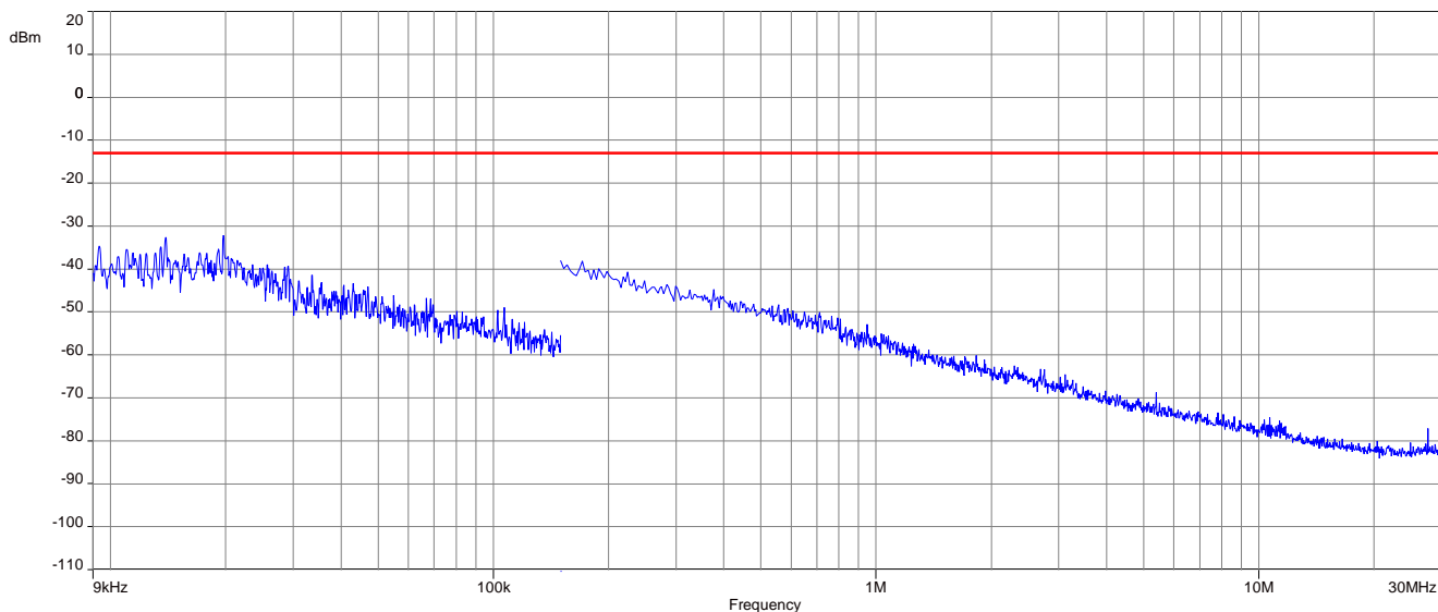
Plot 7: 256-QAM - Middle channel (9 kHz - 30 MHz)
