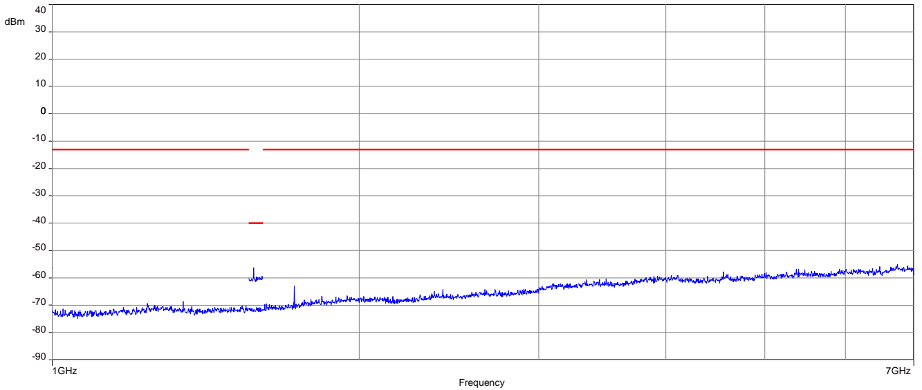
Plot 3: BPSK - Middle channel (1 GHz – 7 GHz)
