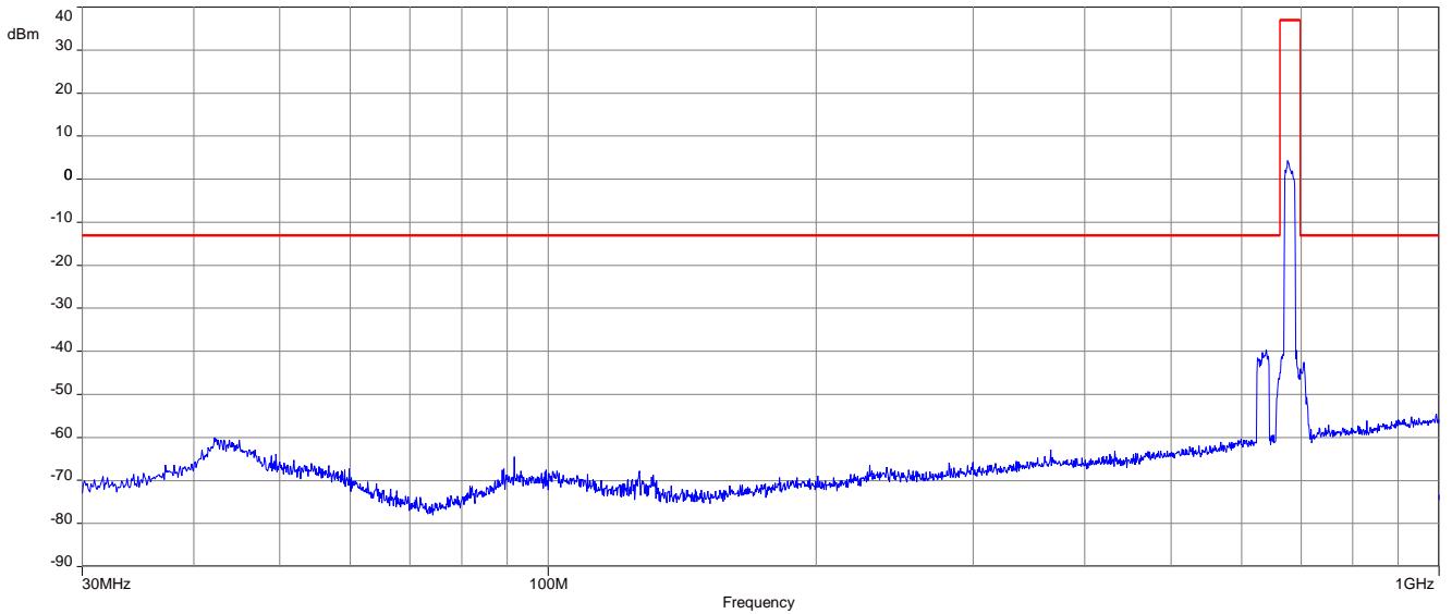
Plot 5: QPSK - Middle channel (30 MHz – 1 GHz)
