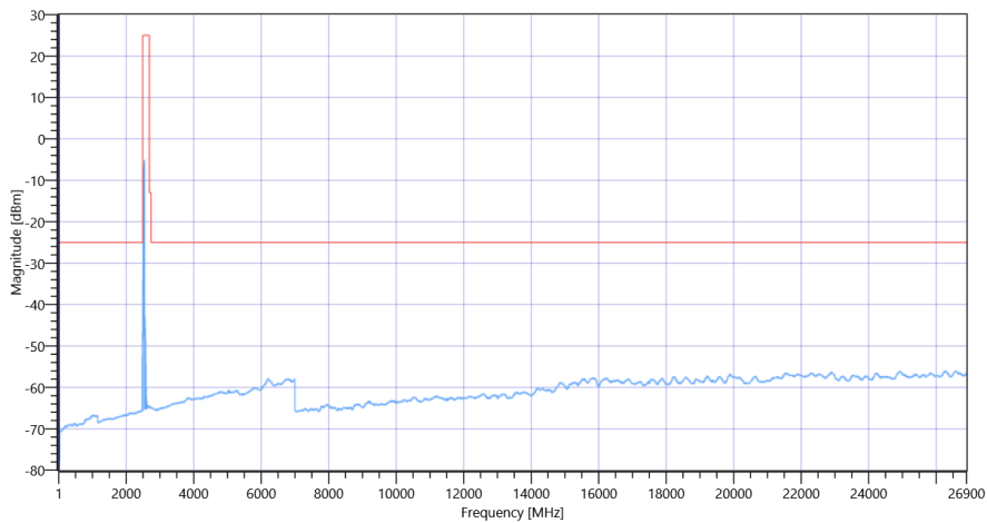
FCC, ISED # TX Emissions conducted ~ NR Band_41 Ant-2 SCS-30 2521.02 MHz
