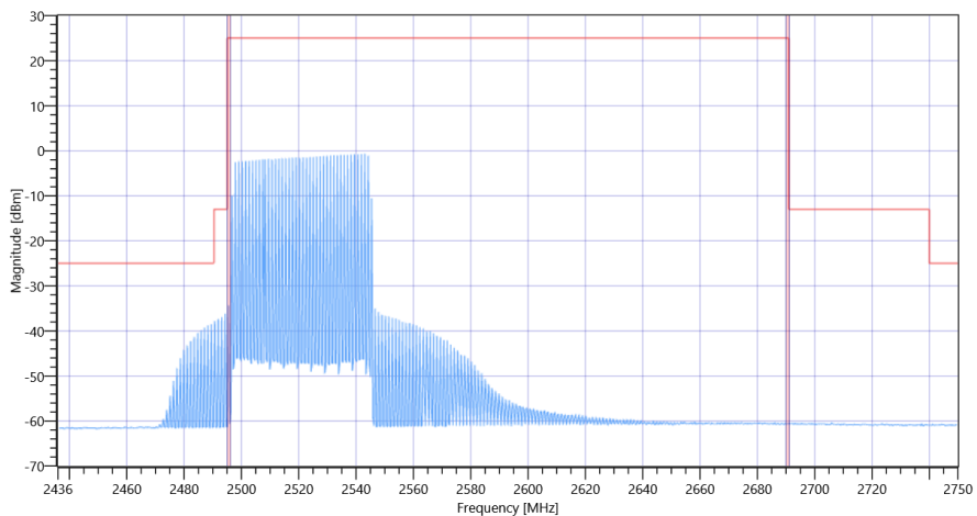
FCC, ISED # TX Emissions conducted ~ NR Band_41 Ant-2 SCS-30 2521.02
