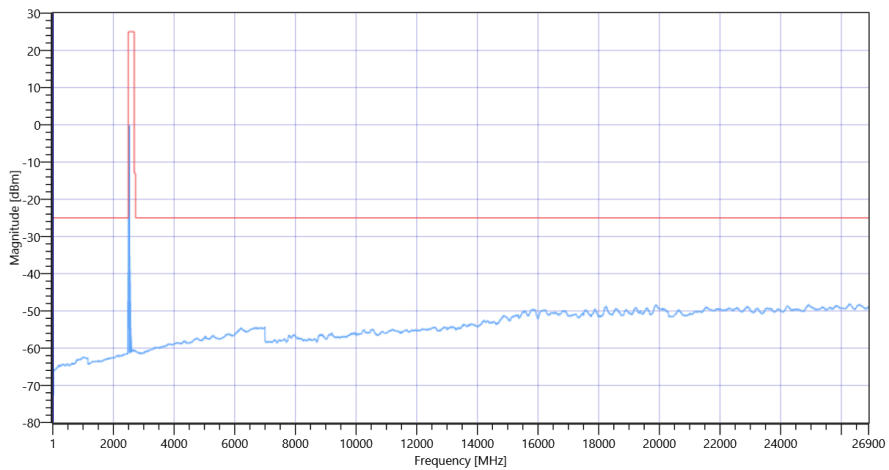
FCC, ISED # TX Emissions conducted ~ NR Band_41 Ant-2 SCS-30 2516.01 MHz
