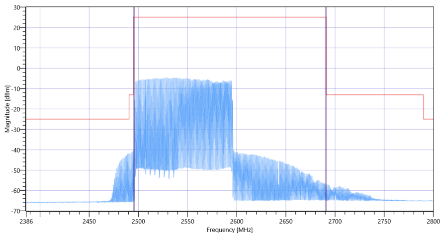
FCC, ISED # TX Emissions conducted ~ NR Band_41 Ant-2 SCS-30 2546.01
