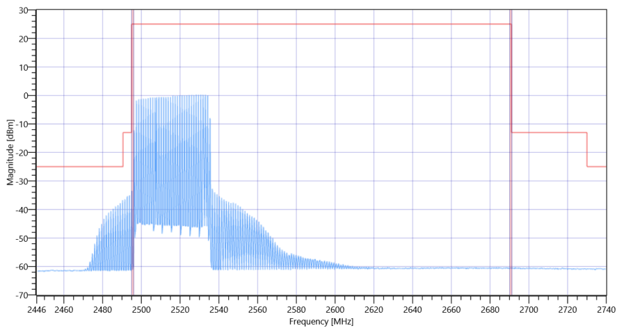
FCC, ISED # TX Emissions conducted ~ NR Band_41 Ant-2 SCS-30 2516.01
