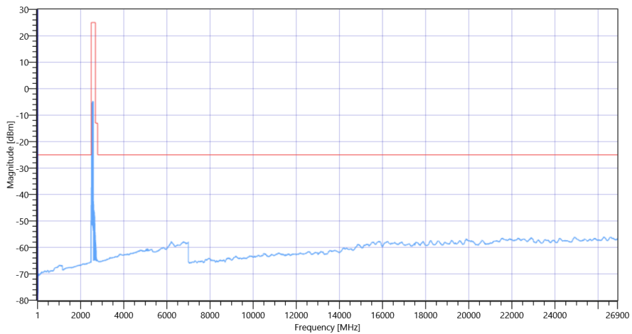
FCC, ISED # TX Emissions conducted ~ NR Band_41 Ant-2 SCS-30 2546.01 MHz
