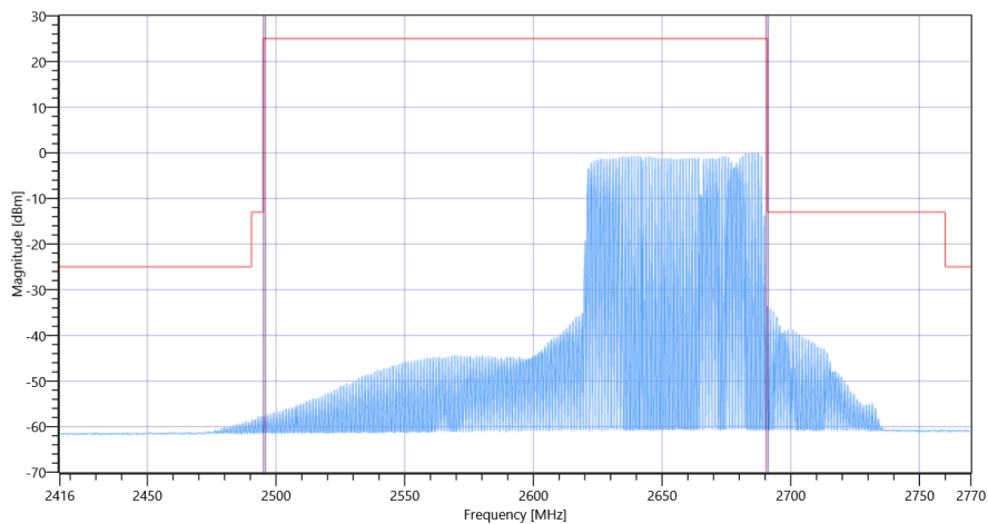
FCC, ISED # TX Emissions conducted ~ NR Band_41 Ant-1 SCS-30 2655
