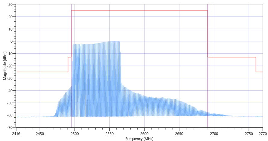
FCC, ISED # TX Emissions conducted ~ NR Band_41 Ant-1 SCS-30 2531.01
