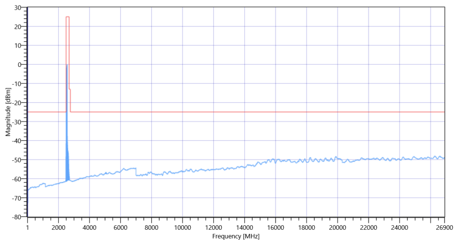
FCC, ISED # TX Emissions conducted ~ NR Band_41 Ant-1 SCS-30 2531.01 MHz
