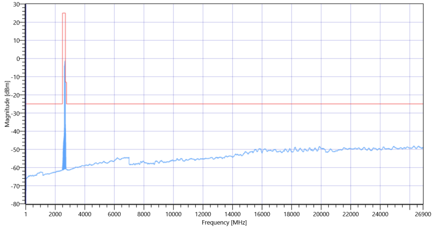
FCC, ISED # TX Emissions conducted ~ NR Band_41 Ant-1 SCS-30 2655 MHz
