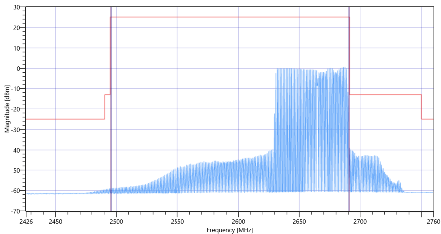
FCC, ISED # TX Emissions conducted ~ NR Band_41 Ant-1 SCS-30 2659.98
