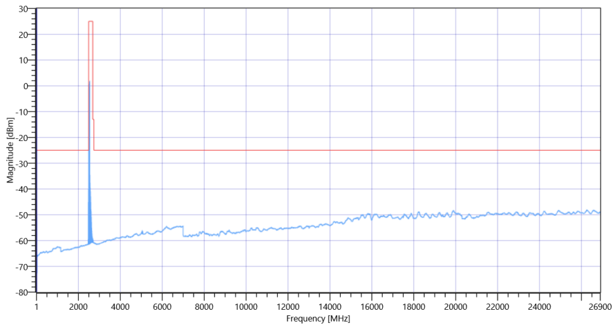
FCC, ISED # TX Emissions conducted ~ NR Band_41 Ant-1 SCS-30 2521.02 MHz
