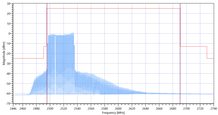
FCC, ISED # TX Emissions conducted ~ NR Band_41 Ant-1 SCS-30 2516.01
