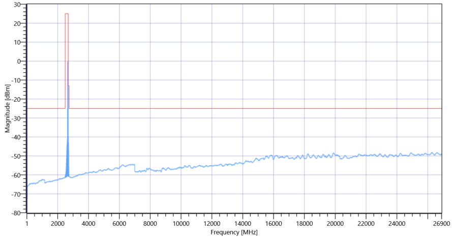
FCC, ISED # TX Emissions conducted ~ NR Band_41 Ant-1 SCS-30 2664.99 MHz
