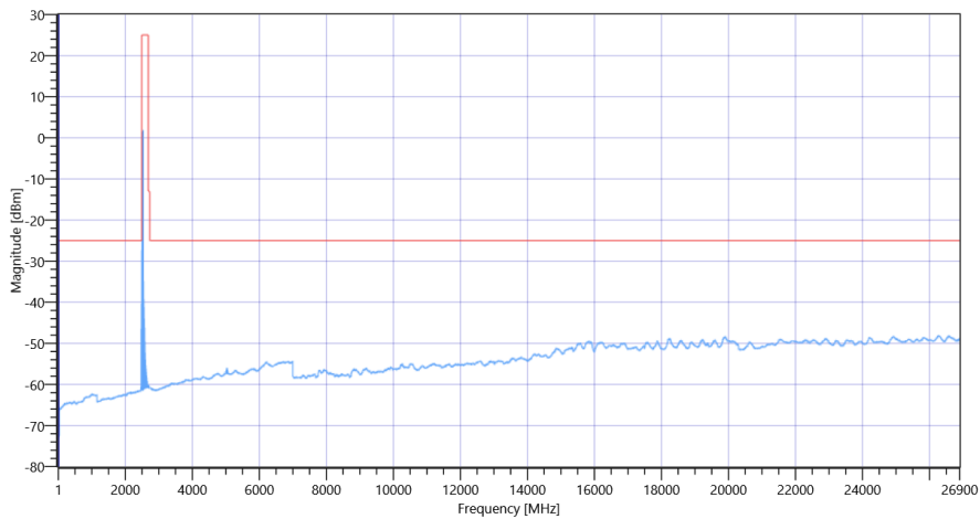
FCC, ISED # TX Emissions conducted ~ NR Band_41 Ant-1 SCS-30 2516.01 MHz
