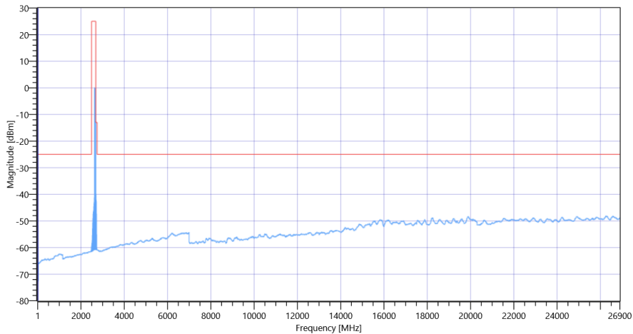
FCC, ISED # TX Emissions conducted ~ NR Band_41 Ant-1 SCS-30 2659.98 MHz
