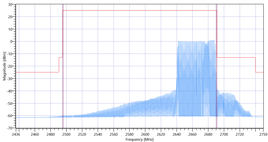
FCC, ISED # TX Emissions conducted ~ NR Band_41 Ant-1 SCS-30 2664.99
