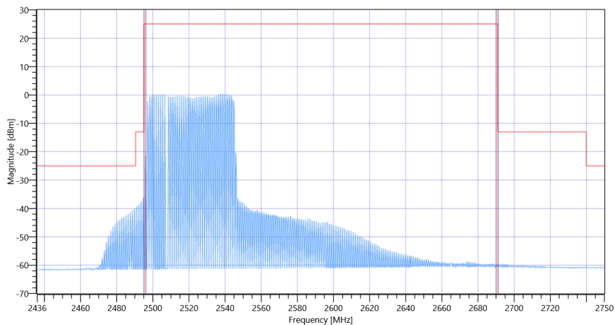
FCC, ISED # TX Emissions conducted ~ NR Band_41 Ant-1 SCS-30 2521.02
